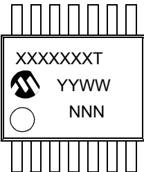
14-Lead TSSOP
