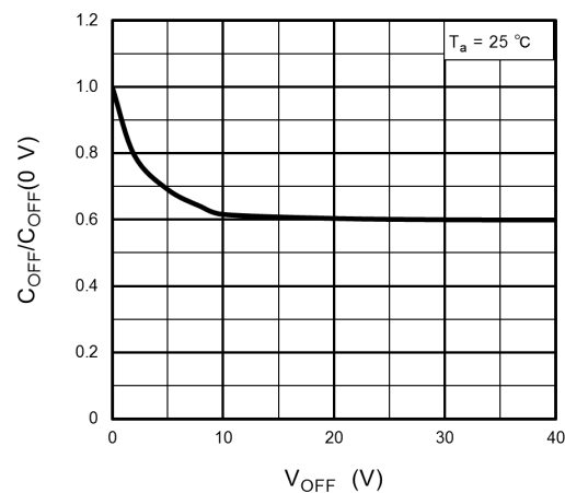
Fig. 12.10 C_{OFF}/C_{OFF}(0 V) - V_{OFF}
