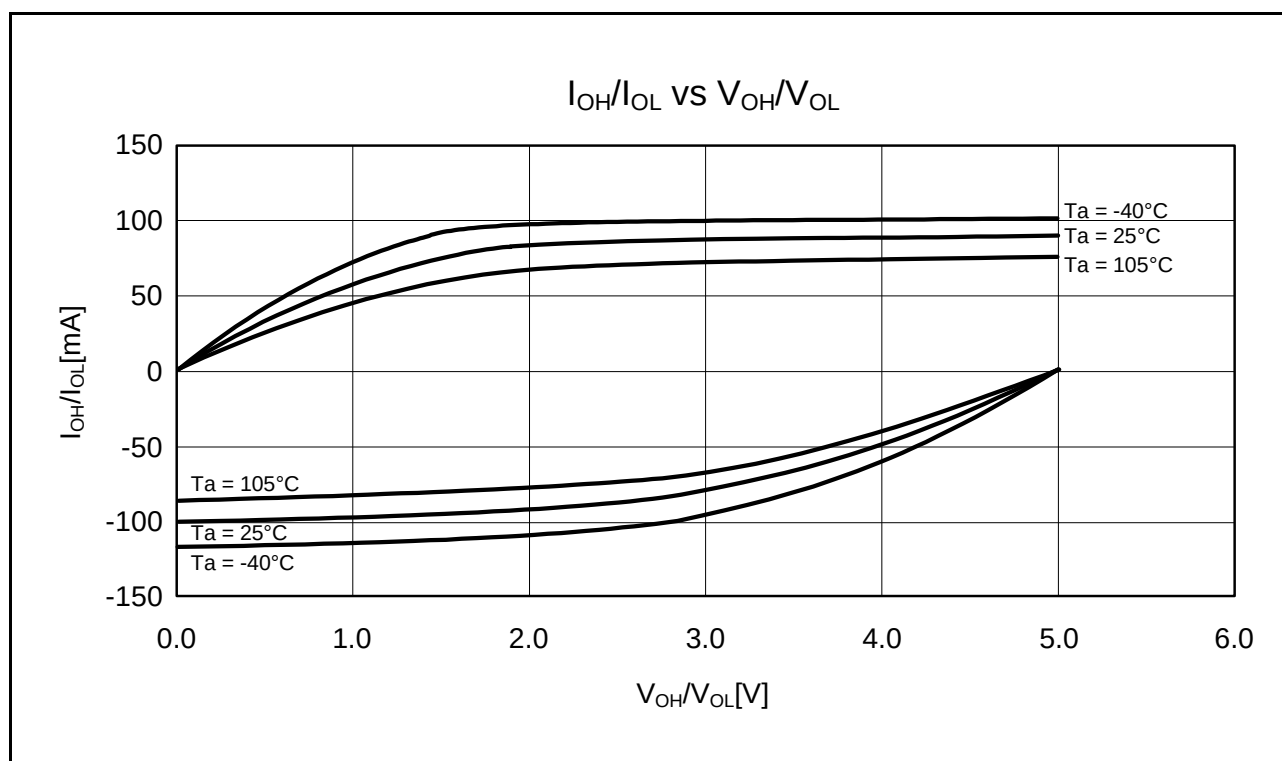
Figure 5.10 V_{OH}/V_{OL} and I_{OH}/I_{OL} Temperature Characteristics at V_{CC} = 5.0 \text{ V} when Normal Output is Selected (Reference Data)
