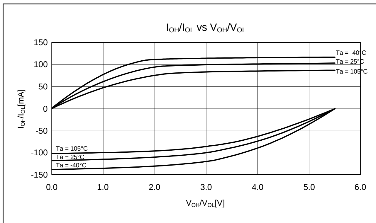
Figure 5.11 V_{OH}/V_{OL} and I_{OH}/I_{OL} Temperature Characteristics at V_{CC} = 5.5 \text{ V} when Normal Output is Selected (Reference Data)
