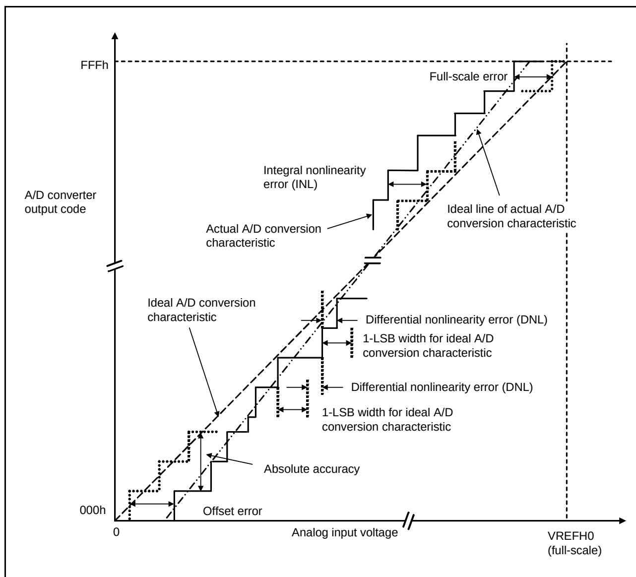
Figure 5.48 Illustration of A/D Converter Characteristic Terms
