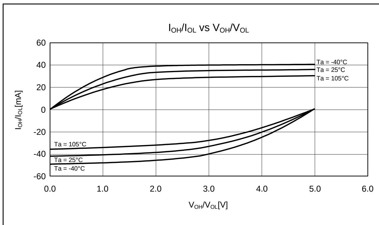
Figure 5.6 V_{OH}/V_{OL} and I_{OH}/I_{OL} Temperature Characteristics at V_{CC} = 5.0 \text{ V} when Normal Output is Selected (Reference Data)
