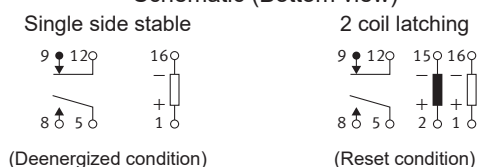
Schematic (Bottom view)
