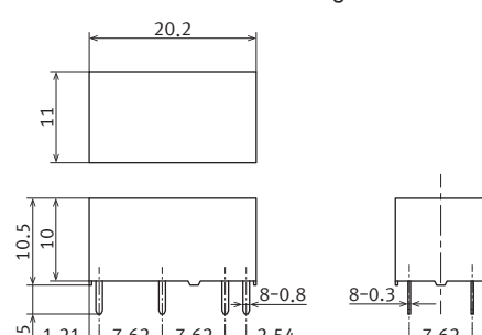
2 coil latching
