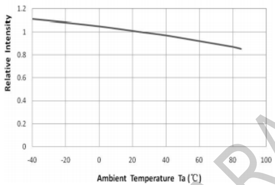
Relative Intensity VS. Ambient Temperature (Ta=25°C)
