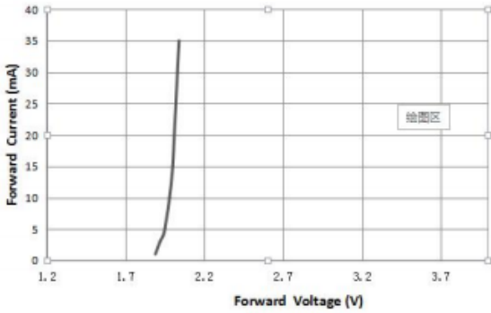
Forward Current VS. Forward Voltage (Ta=25°C)
