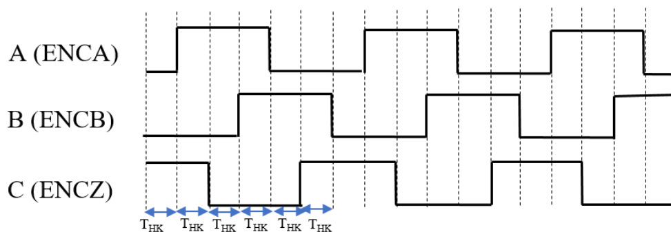
Figure 3.11-40: Hall Timing Diagram
