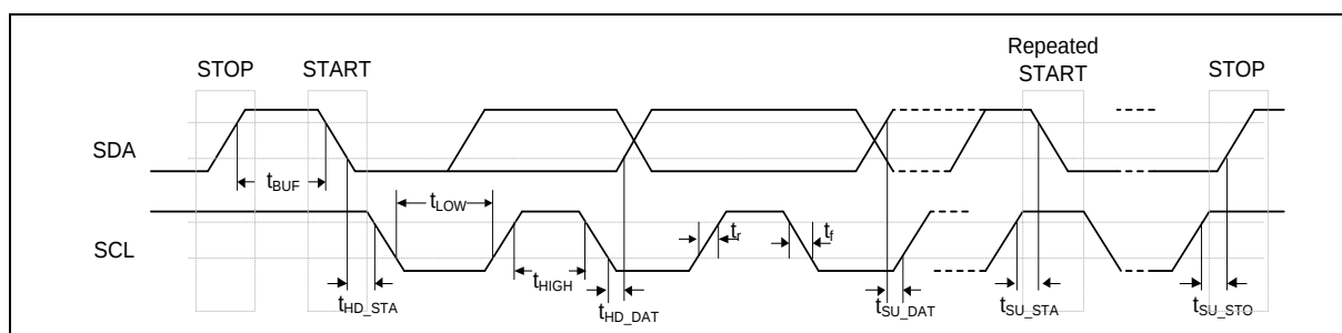
Figure 2.26-1: I 2 C Bus Timing
