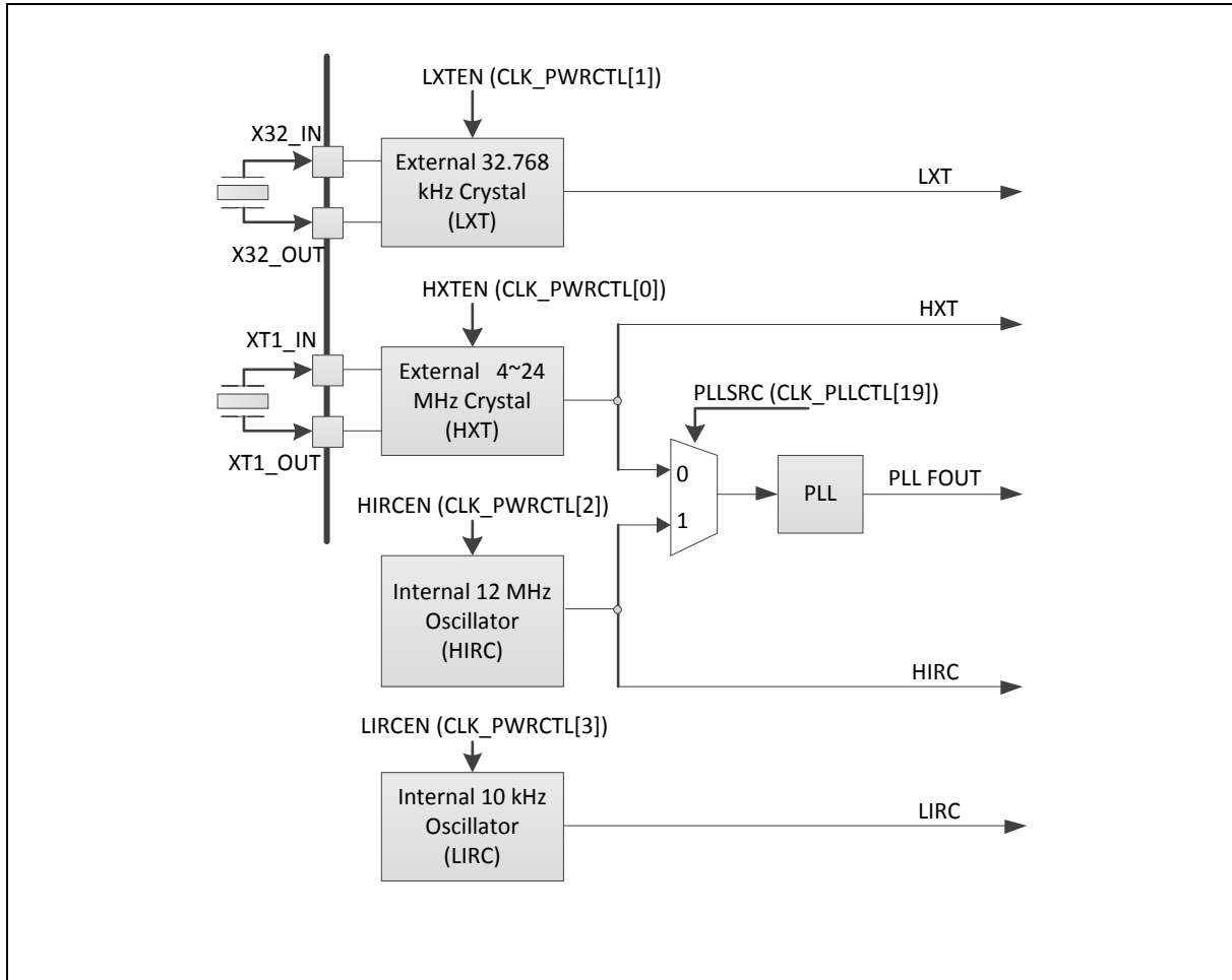
Figure 2.3-2: Clock Generator Block Diagram
