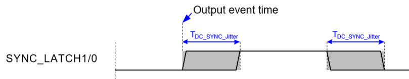
Figure 3.11-21: SYNC timing
