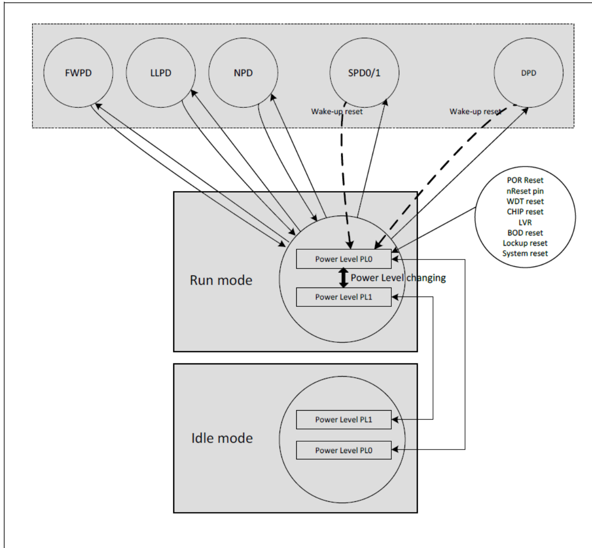
Figure 2.2-8: Power Distribution Diagram
