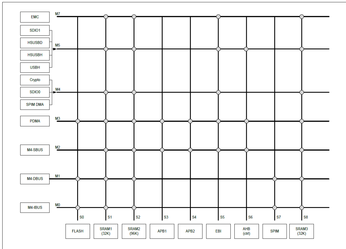
Figure 2.2-11: AX58200 Bus Matrix Diagram
