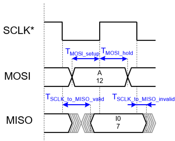
Figure 3.11-26: Basic MOSI/MISO timing
