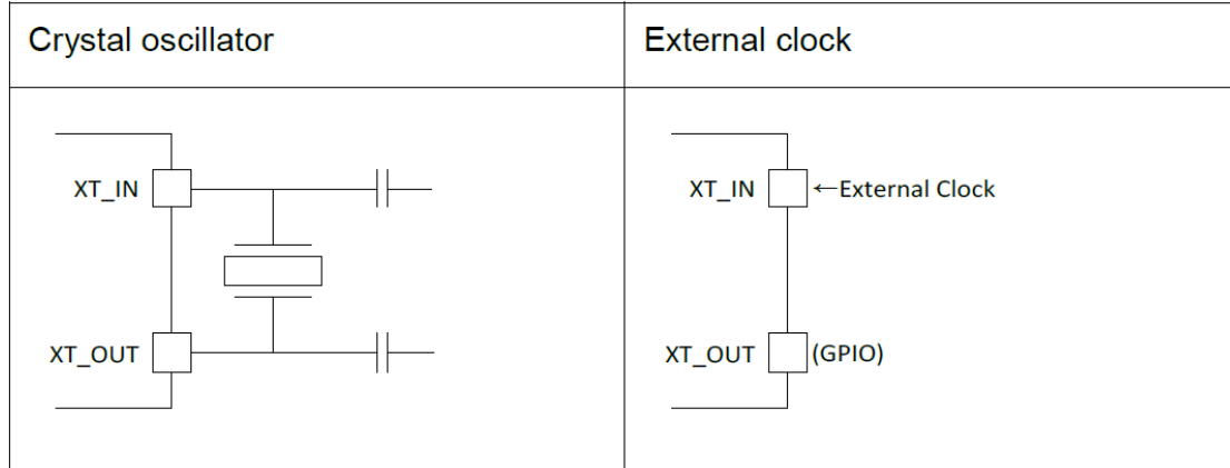
Figure 2.3-8: HXT Clock Sources
