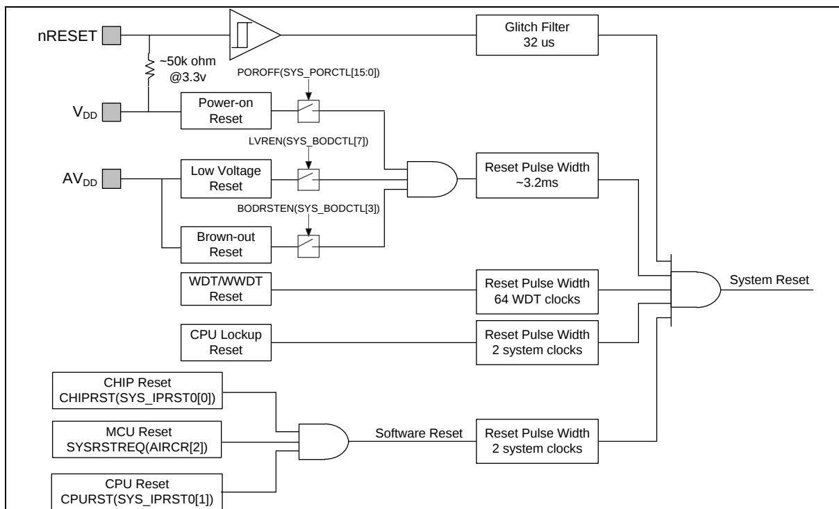
Figure 2.2-1: System Reset Sources
