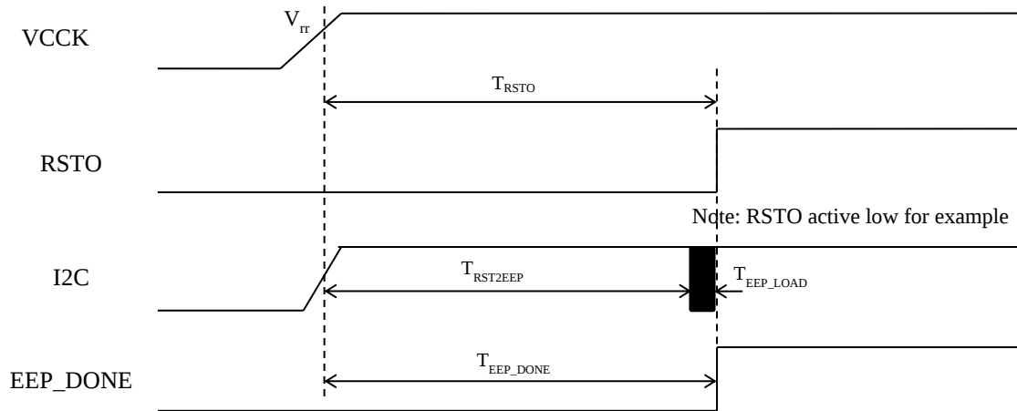
Figure 3.11-46: Power up to RSTO, EEPROM and EEP_DONE Timing
