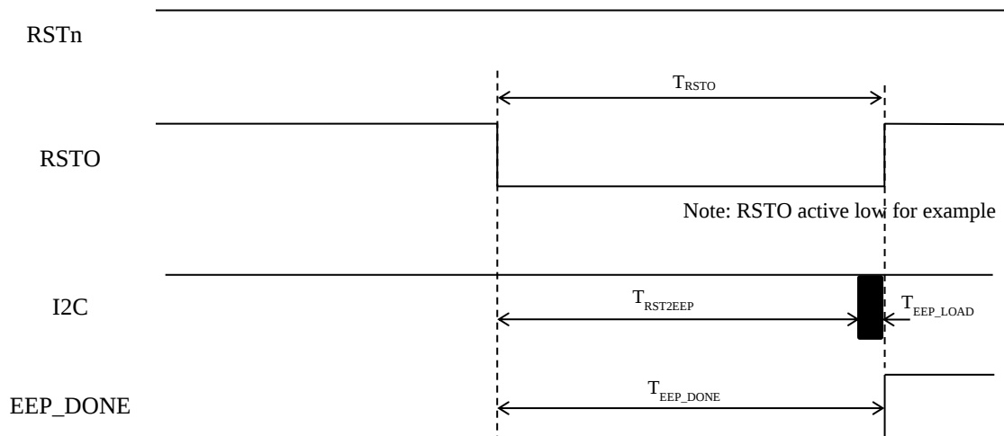
Figure 3.11-48: Register Reset to RSTO, EEPROM and EEP_DONE Timing
