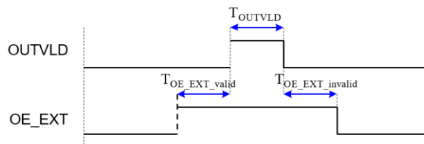
Figure 3.11-25: OE_EXT timing
