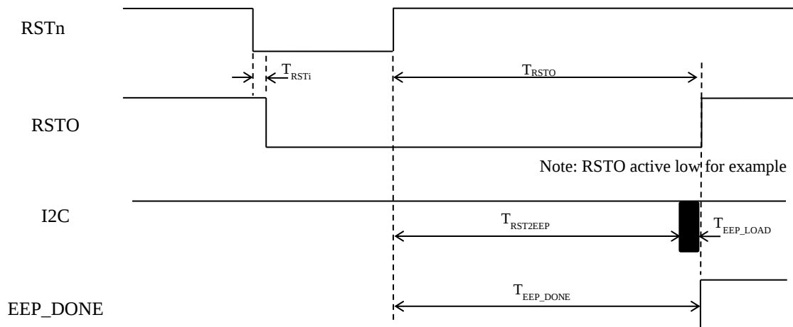
Figure 3.11-47: RSTn to RSTO, EEPROM and EEP_DONE Timing
