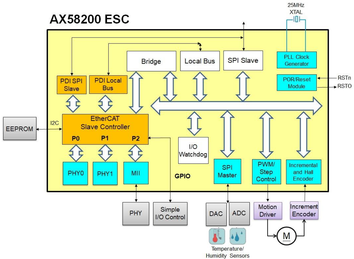
Figure 2.41-1: ESC Sub-system Block Diagram
