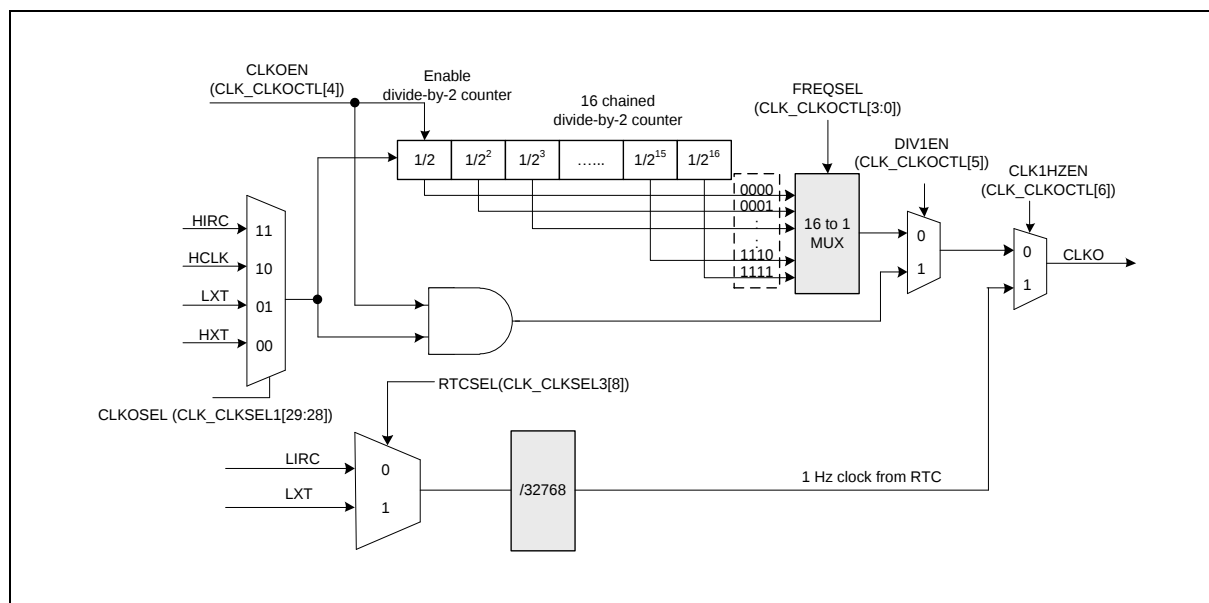
Figure 2.3-6: Clock Output Block Diagram
