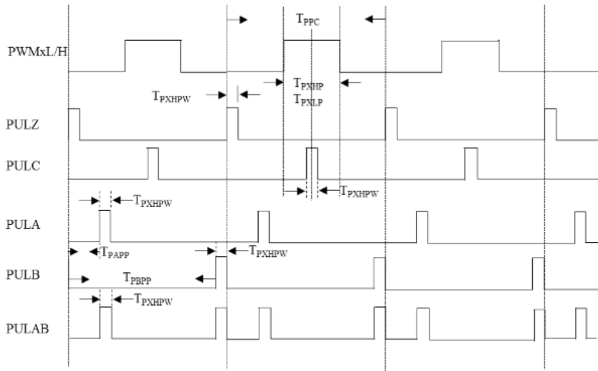
Figure 3.11-33: PWMx Timing
