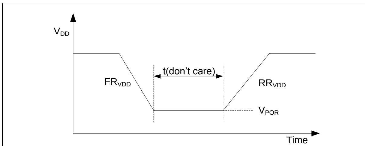
Figure 3.5-1: Power-up Ramp Condition
