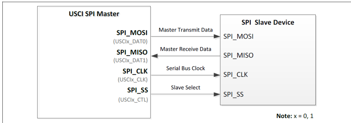
Figure 2.25-1: SPI Master Mode Application Block Diagram
