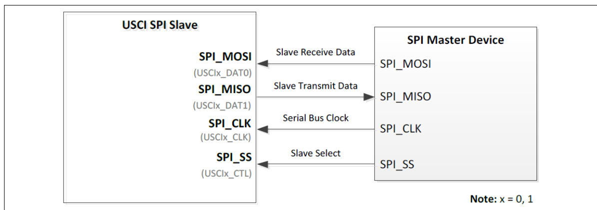
Figure 2.25-2: SPI Slave Mode Application Block Diagram
