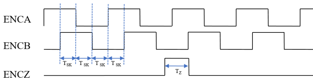
Figure 3.11-37: ABZ Timing Diagram
