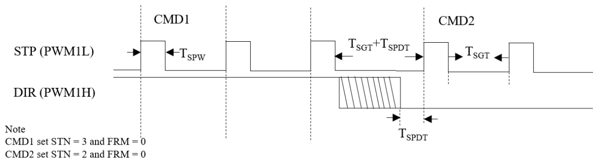
Figure 3.11-36: One Shot with multi Step Timing Diagram
