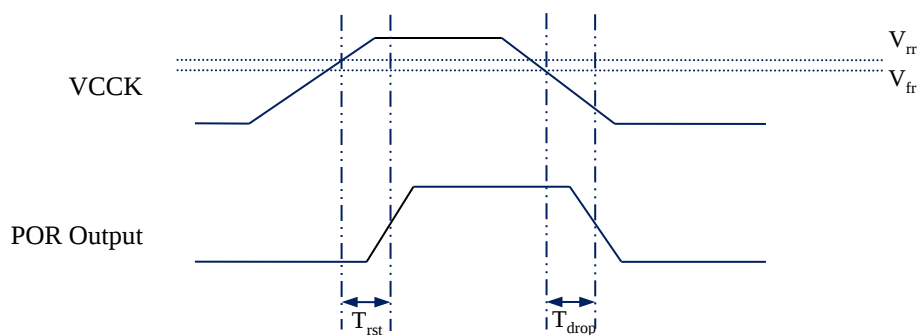
Figure 3.5-2: Power On Reset (POR) Timing Diagram
