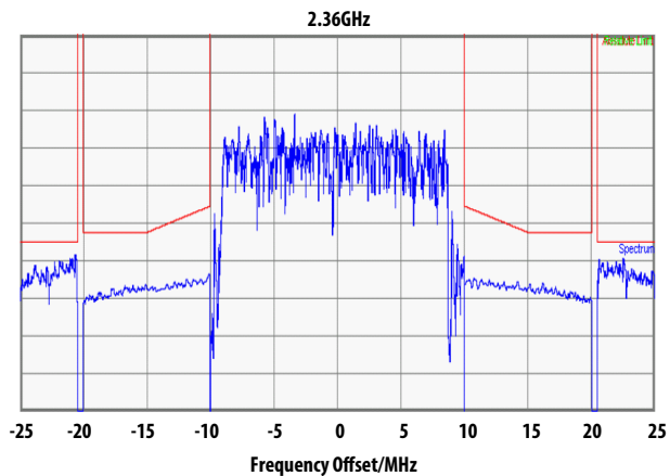
Figure 35. Spectrum Emission Mask 29.0dBm @ 2.36GHz
