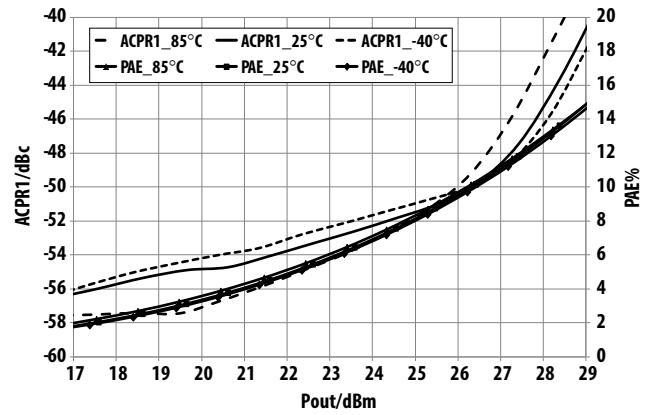
Figure 17. Over-temperature ACPR1, PAE vs. P_{out} @ 2.39 GHz V_{dd}=V_{ddBias}=5.5 V operating voltage
