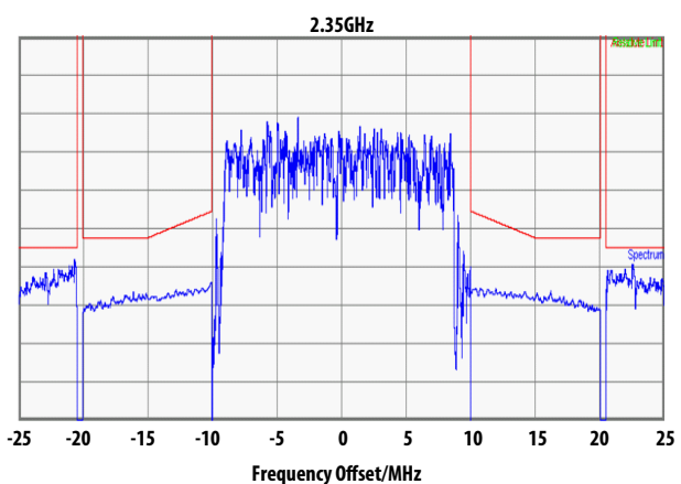
Figure 34. Spectrum Emission Mask 29.0dBm @ 2.35GHz
