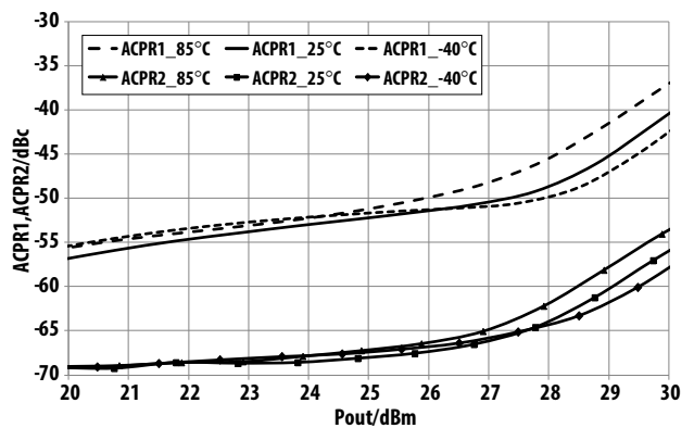
Figure 19. Over-temperature ACPR1, ACPR2 vs. P_{out} @ 2.35 GHz V_{dd}=V_{ddBias}=5.5 V operating voltage
