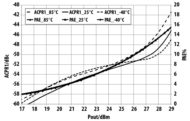
Figure 15. Over-temperature ACPR1, PAE vs. P_{out} @ 2.35 GHz V_{dd}=V_{ddBias}=5.5 V operating voltage
