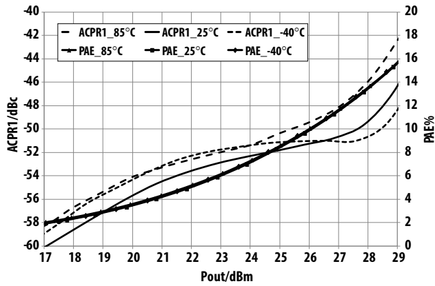
Figure 14. Over-temperature ACPR1, PAE vs. P_{out} @ 2.33 GHz V_{dd}=V_{ddBias}=5.5 V operating voltage
