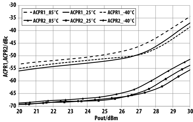
Figure 18. Over-temperature ACPR1, ACPR2 vs. P_{out} @ 2.35 GHz V_{dd}=V_{ddBias}=5.0 V operating voltage
