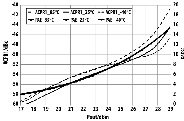
Figure 16. Over-temperature ACPR1, PAE vs. P_{out} @ 2.36 GHz V_{dd}=V_{ddBias}=5.5 V operating voltage
