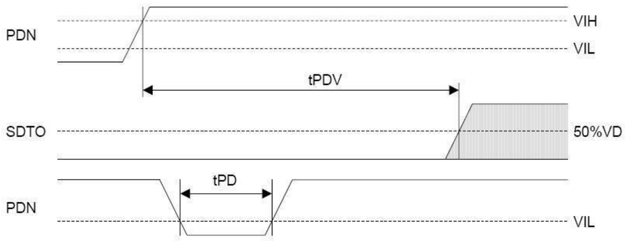
Figure 6. Reset Timing
