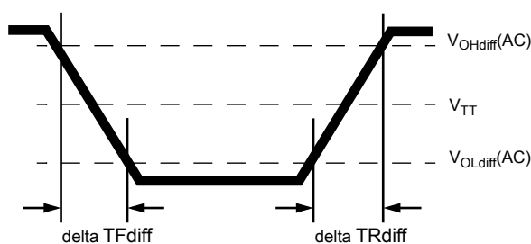
Figure 16. Differential Output Slew Rate Definition
