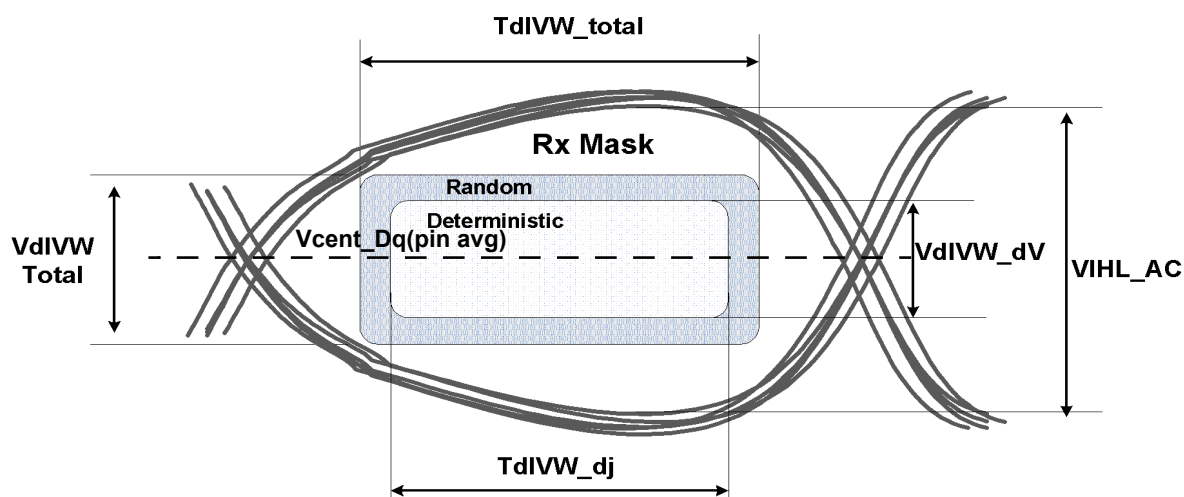
Figure 22. DQ Receiver(Rx) compliance mask
