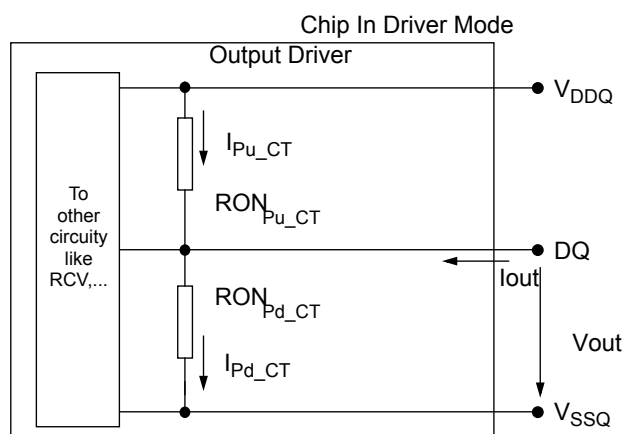
Figure 14. Output Driver
