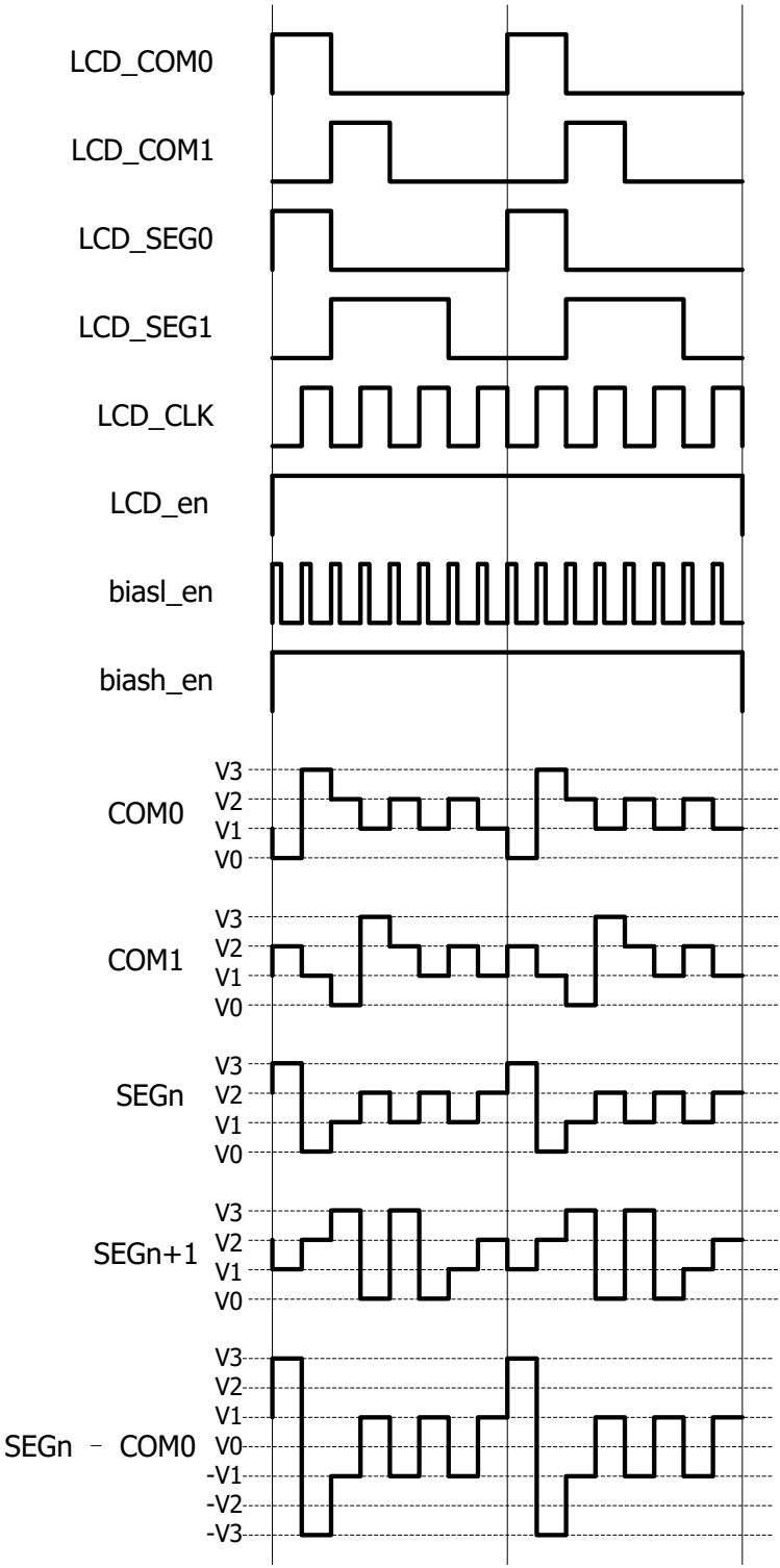
图 31-2LCD 驱动波形(1/4 duty, 1/3 bias, type A)
