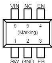
Figure 1. Pin Assignment of FP6745
