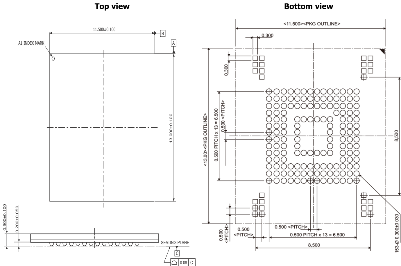
[Figure 3] 11.5mm x13.0mm x 1.0mm Package dimension
