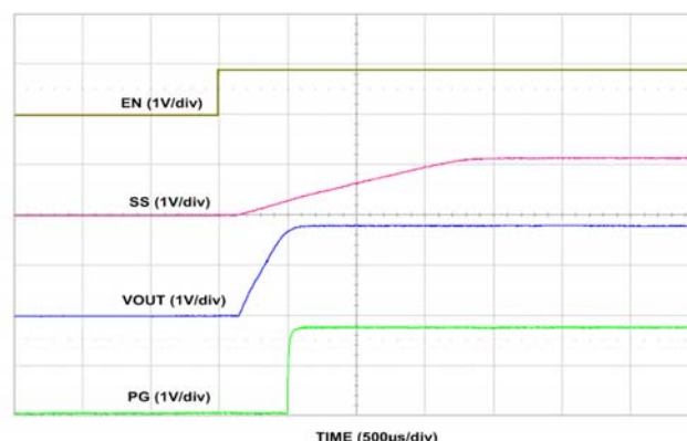
FIGURE 18. ENABLE START-UP
