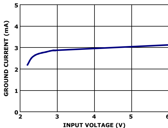
FIGURE 10. GROUND CURRENT vs SUPPLY VOLTAGE
