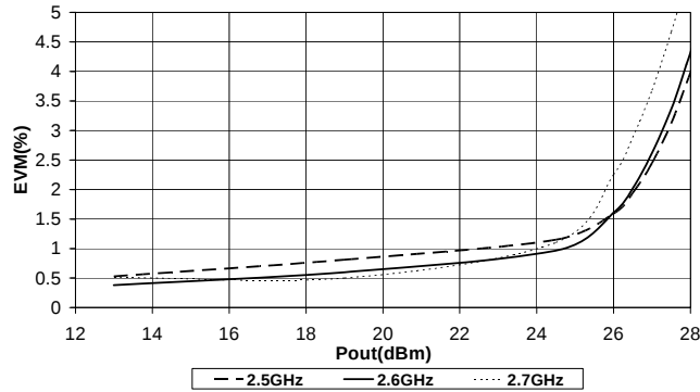
EVM vs Pout F=2.7GHz 802.11g, OFDM 54Mb/S, 64QAM
