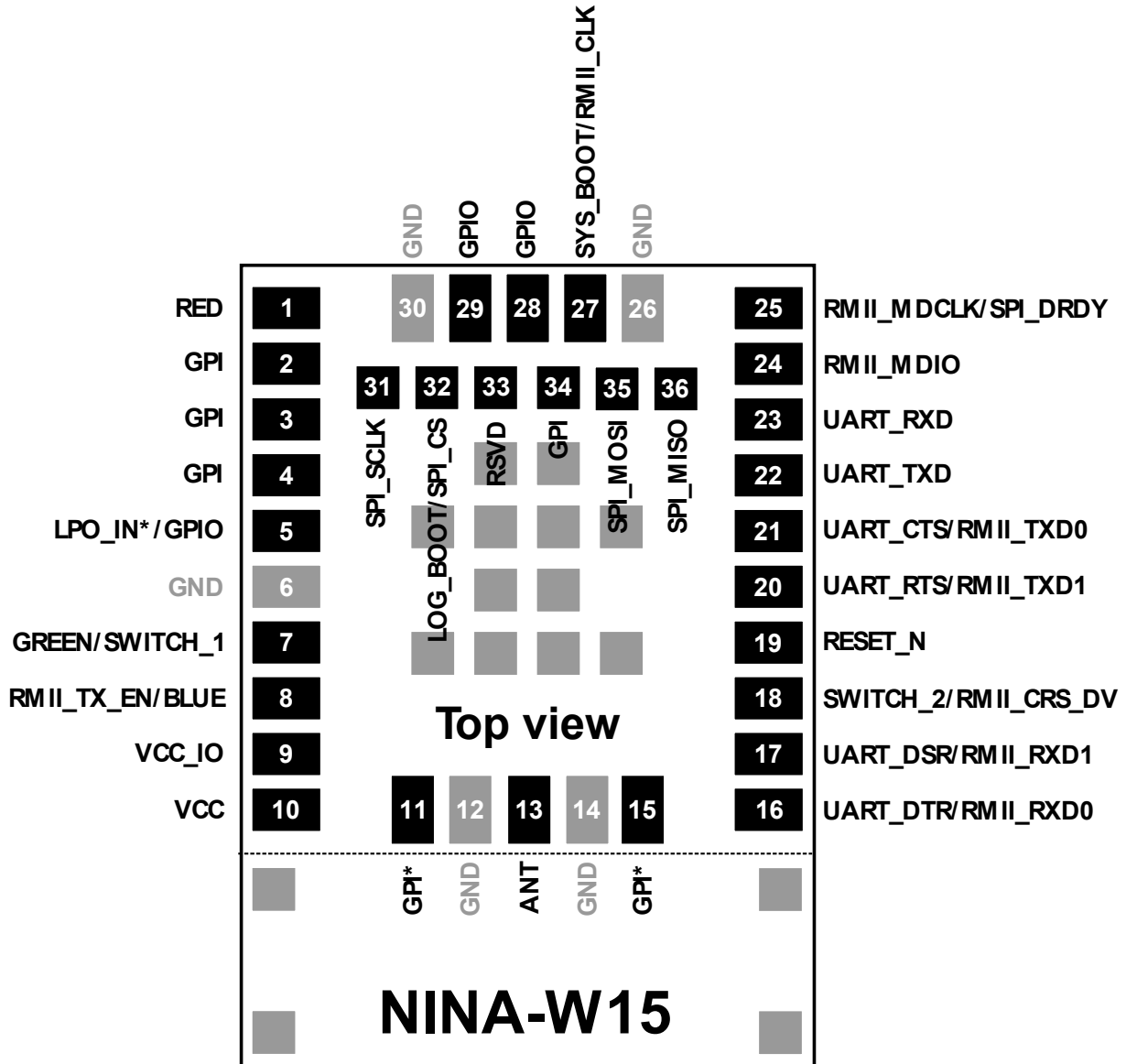
Figure 4: NINA-W15 pin assignment (top view)
