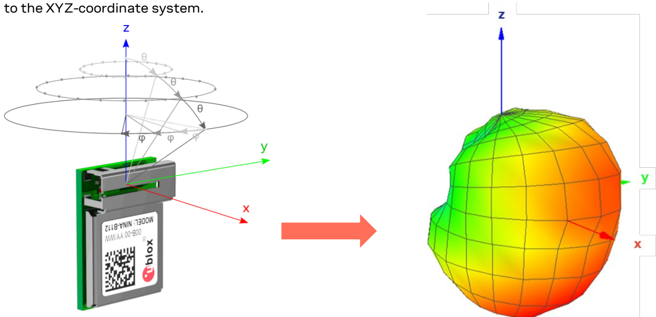
Figure 5: Measurement procedure for determining radiation patterns. A measurement is taken at every dot in the figure to the left and is represented as a grid point in the radiation pattern to the right.
