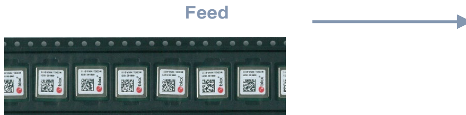
Figure 12: Orientation of NINA-W151 module on tape
