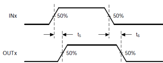
ENx = 1, Resistive Load to GND
