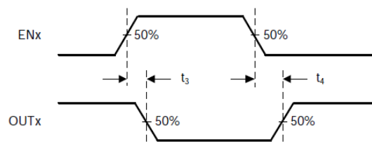
INx = 0, Resistive Load to VM
