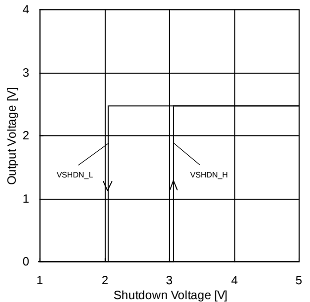
Figure 24. Shutdown Voltage vs Output Voltage ( V_{DD}=5V , A_v=0dB , V_{IN}=2.5V )
