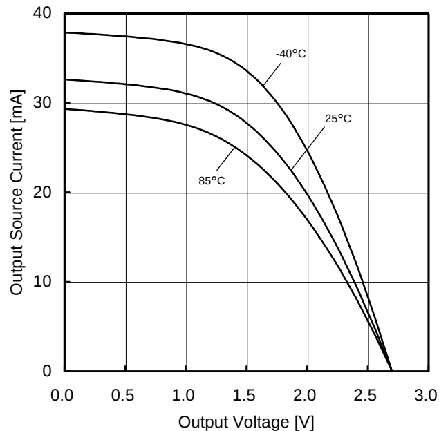
Figure 54. Output Source Current vs Output Voltage ( V_{DD}=2.7V )
