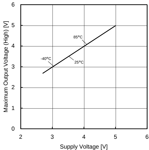
Figure 50. Maximum Output Voltage (High) vs Supply Voltage ( R_L=2k\Omega )
