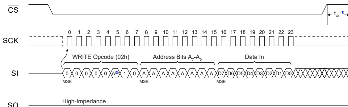
Figure 8-1. Byte Write
