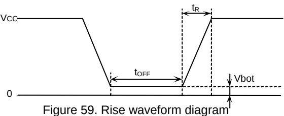
Figure 59. Rise waveform diagram
