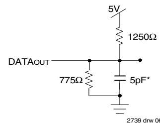
Figure 2. Output Test Load (5pF for tLZ, tHZ, tWZ, tOW) *Including scope and jig.
