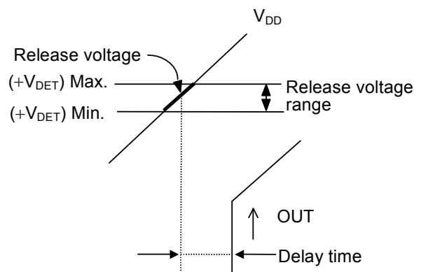
Figure 15 Release Voltage
