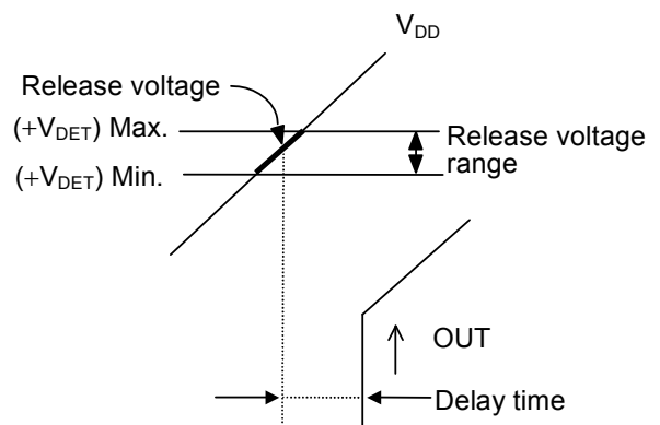
Figure 15 Release Voltage
