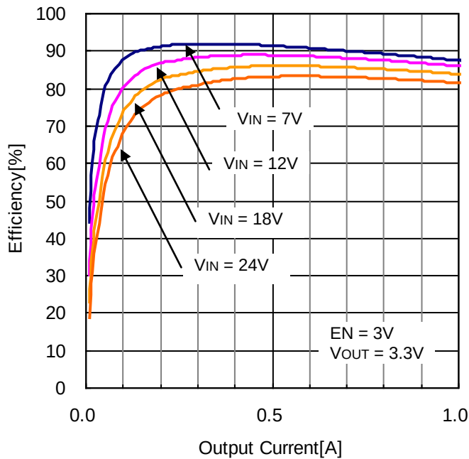
Figure 18. Efficiency vs Output Current (VOUT = 3.3V, L=10μH)
