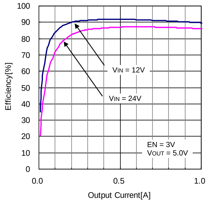
Figure 19. Efficiency vs Output Current (VOUT = 5.0V, L=10μH)
