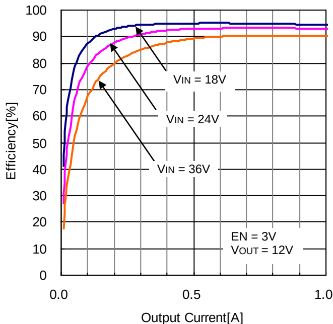
Figure 20. Efficiency vs Output Current (VOUT = 12V, L=10μH)
