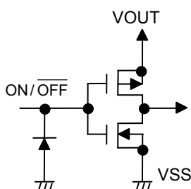
Figure 17 ON/ \overline{\text{OFF}} Pin Structure
