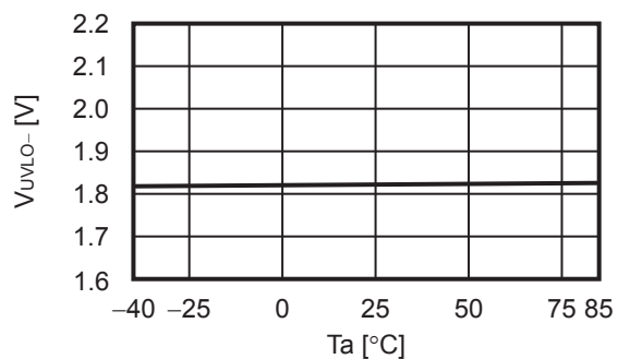
2. 16 UVLO detection voltage ( V_{UVLO-} ) vs. Temperature ( T_a )
