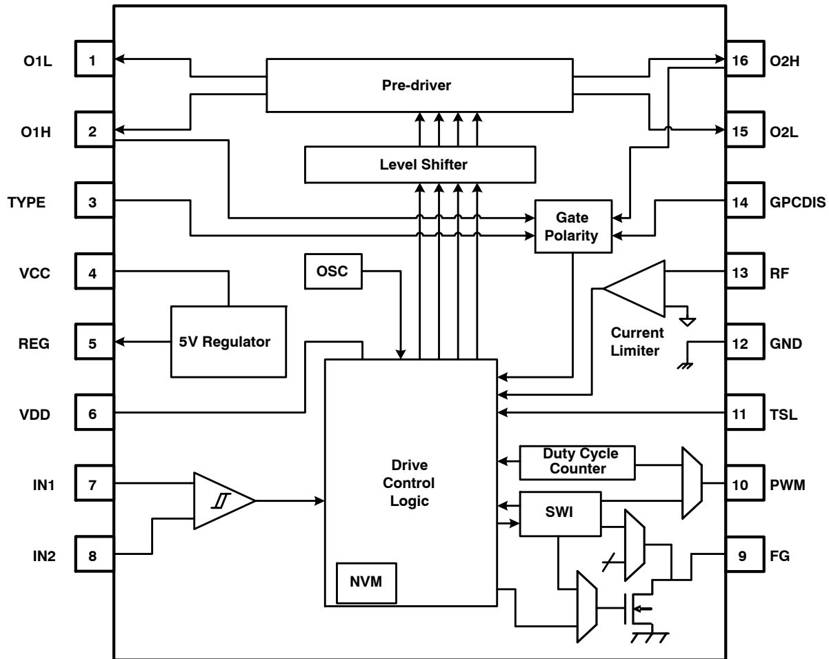
Figure 3. Block Diagram
