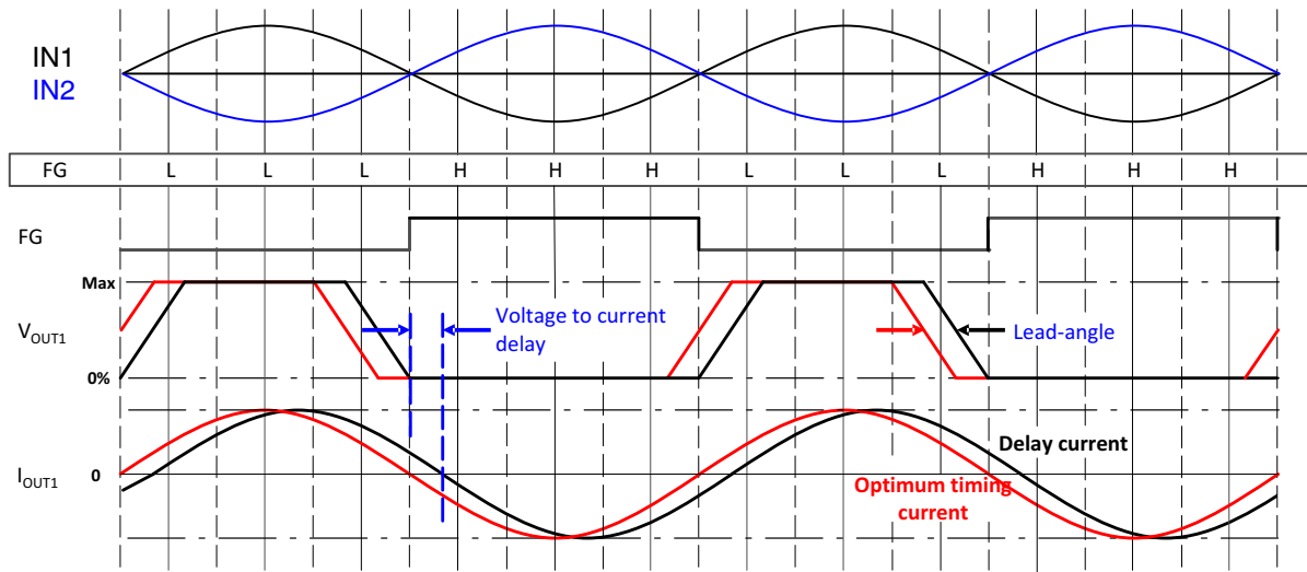
Figure 17. The Relationship Between the Lead-Angle and the Delay of Output Current
