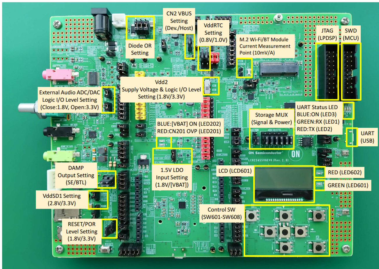
Figure 5. LC823455XGEVK (Detailed, 1/2)
