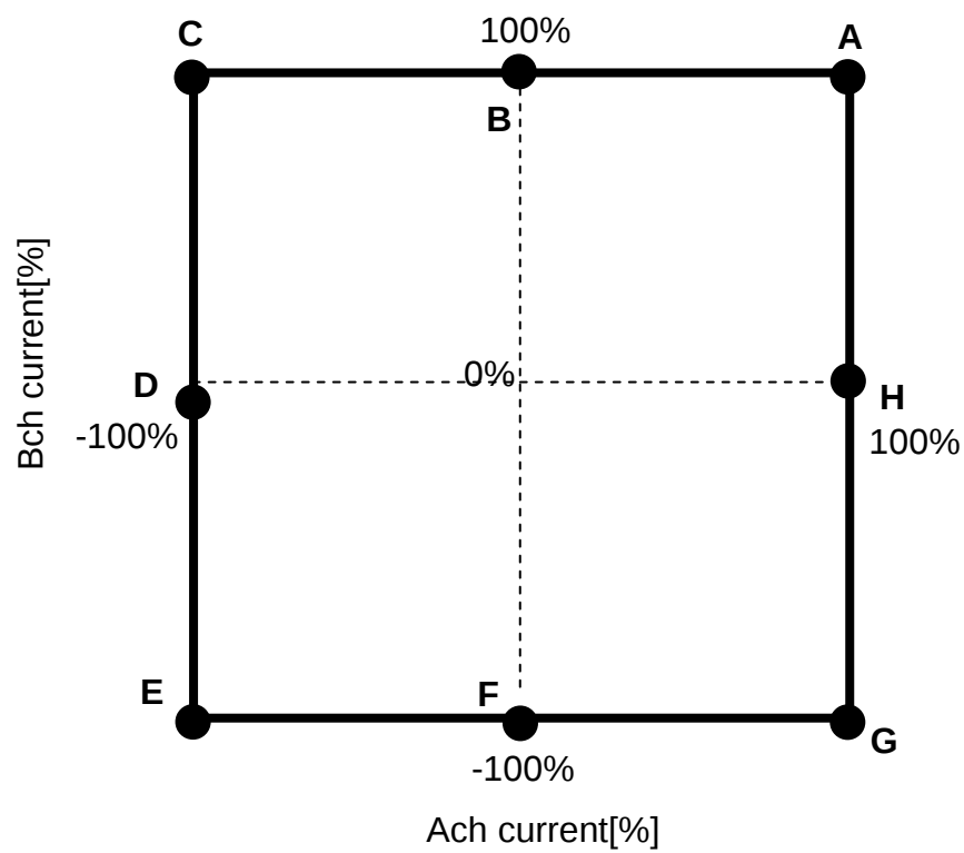
Half step(a) resolution sequence
