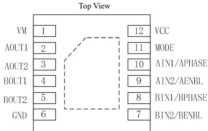
Fig 2. Pad definition of HT8835
