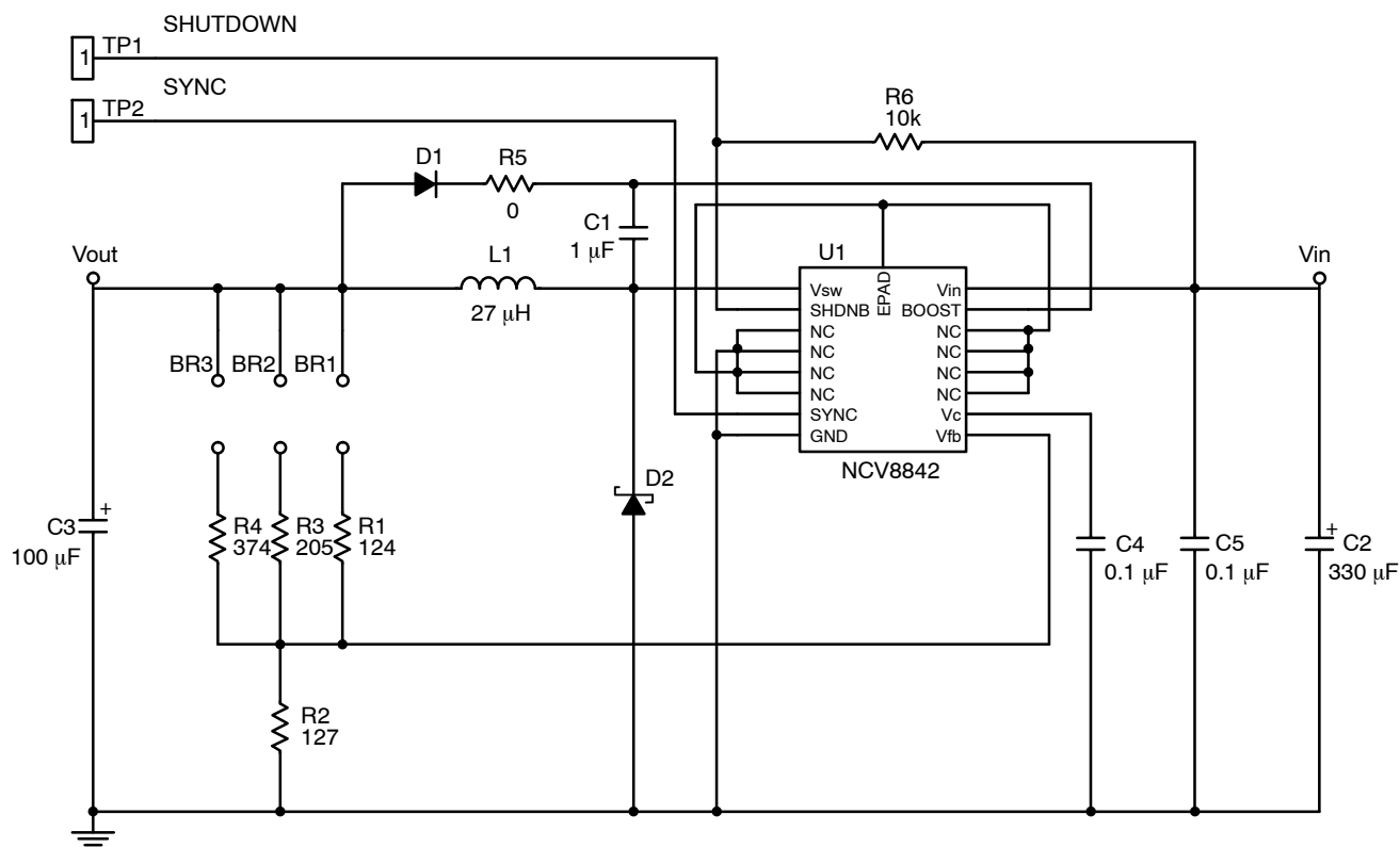
Figure 2. Application Diagram
