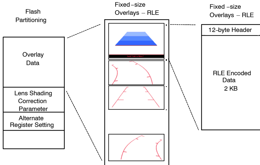
Figure 32. Memory Partitioning
