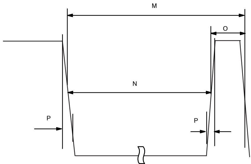
Figure 59. V Pulse
