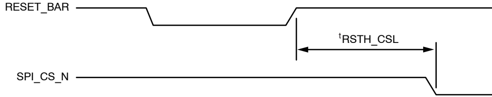
Figure 53. Reset to SPI Access Delay
