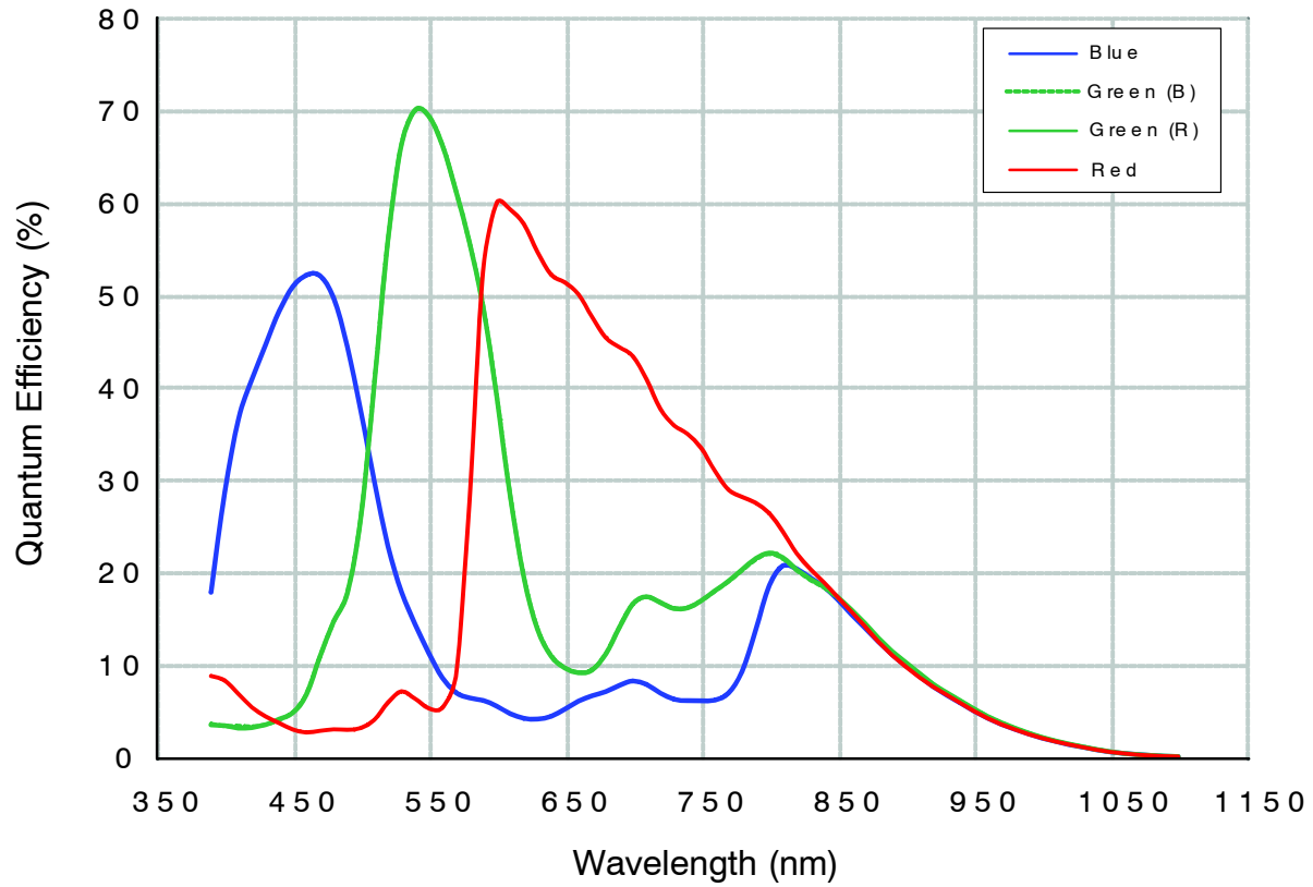
Figure 61. Quantum Efficiency
