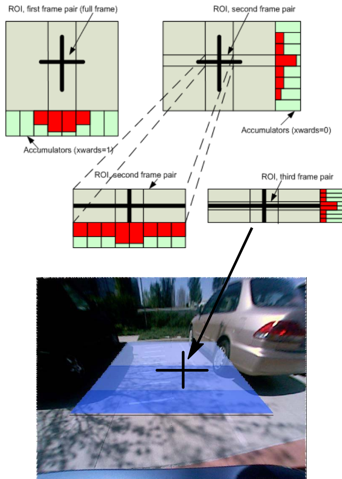
Figure 33. Overlay Calibration
