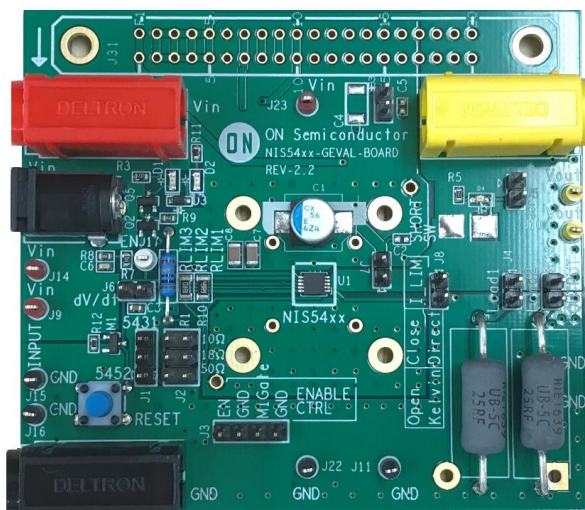
Figure 1: The NIS54xxGEVB evaluation board
