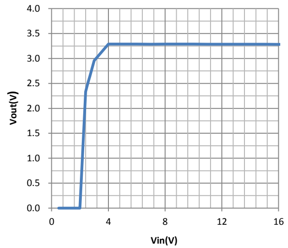
Line Regulation
