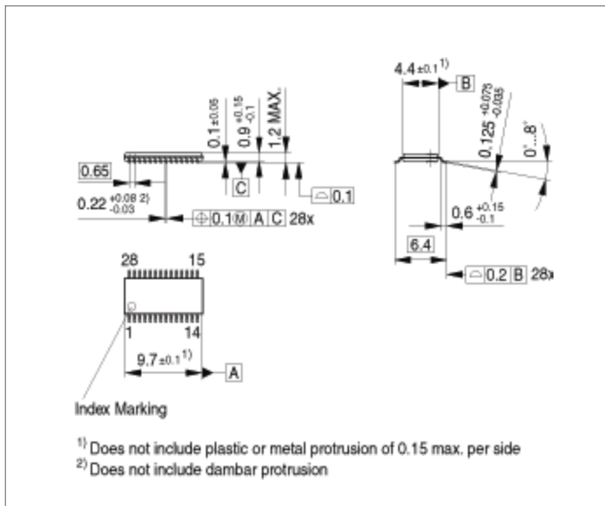
Figure 19 PG-TSSOP-28-12 Package Outline
