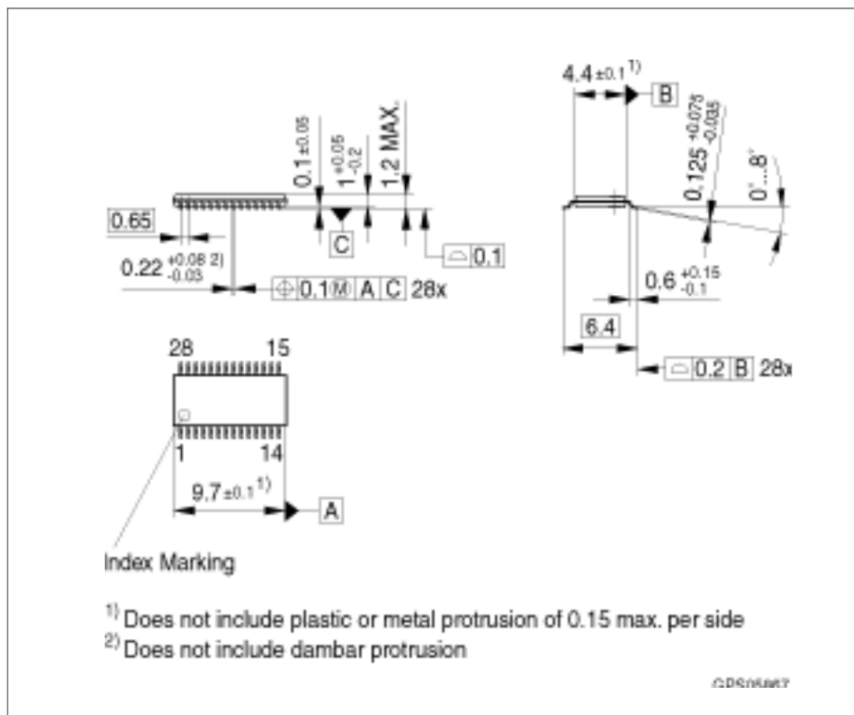
Figure 18 PG-TSSOP-28-1 Package Outline
