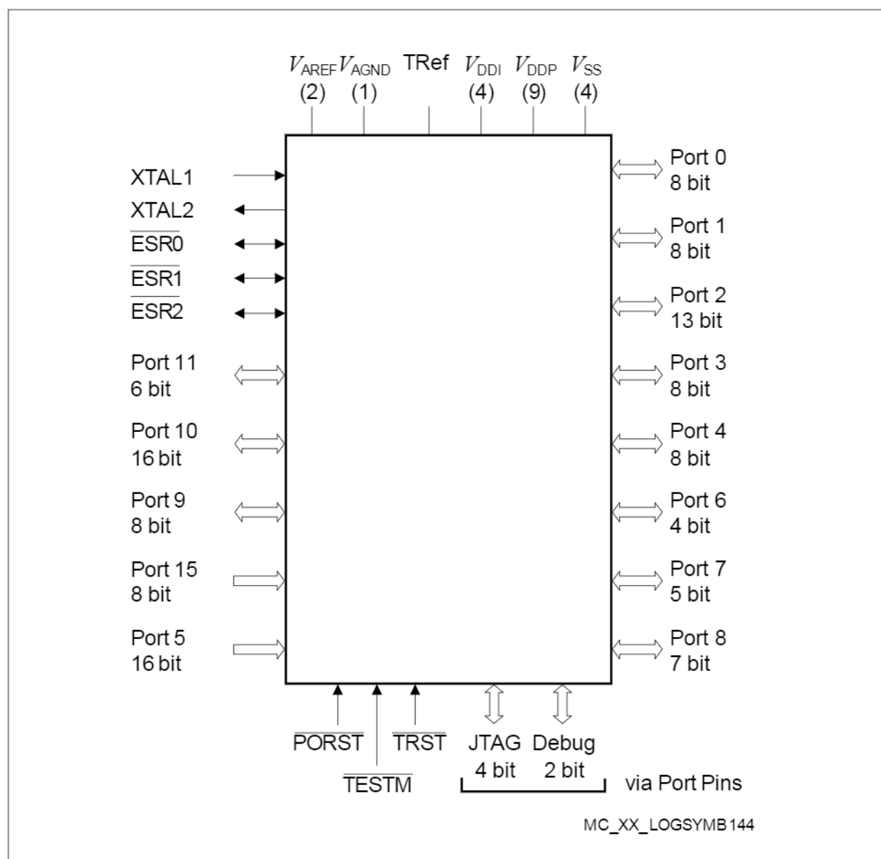
Figure 1 Logic Symbol
