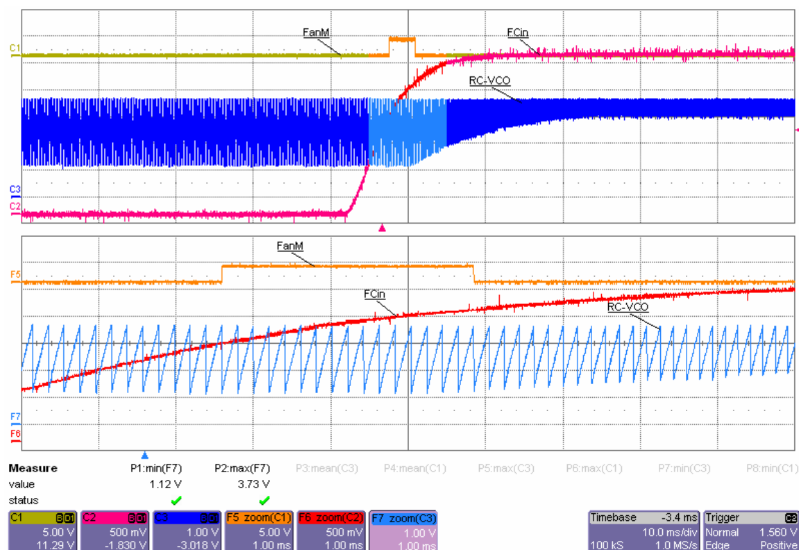
Fig. 5 RC-VCO Valley Voltage At Minimum and Maximum Frequency
