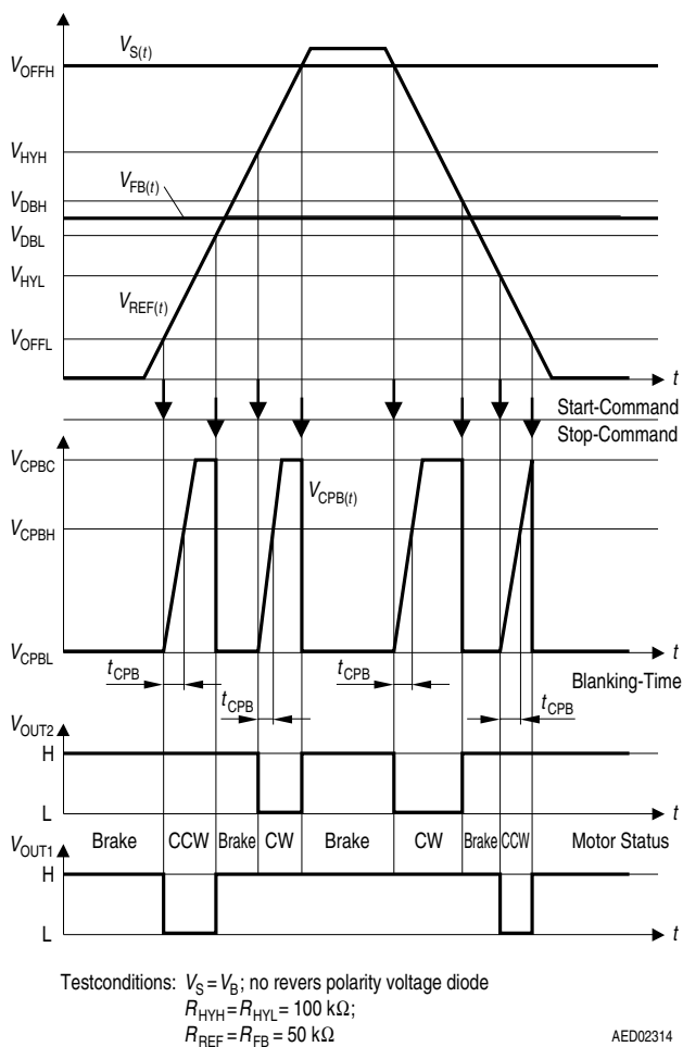
Figure 5 Timing and Phaselag
