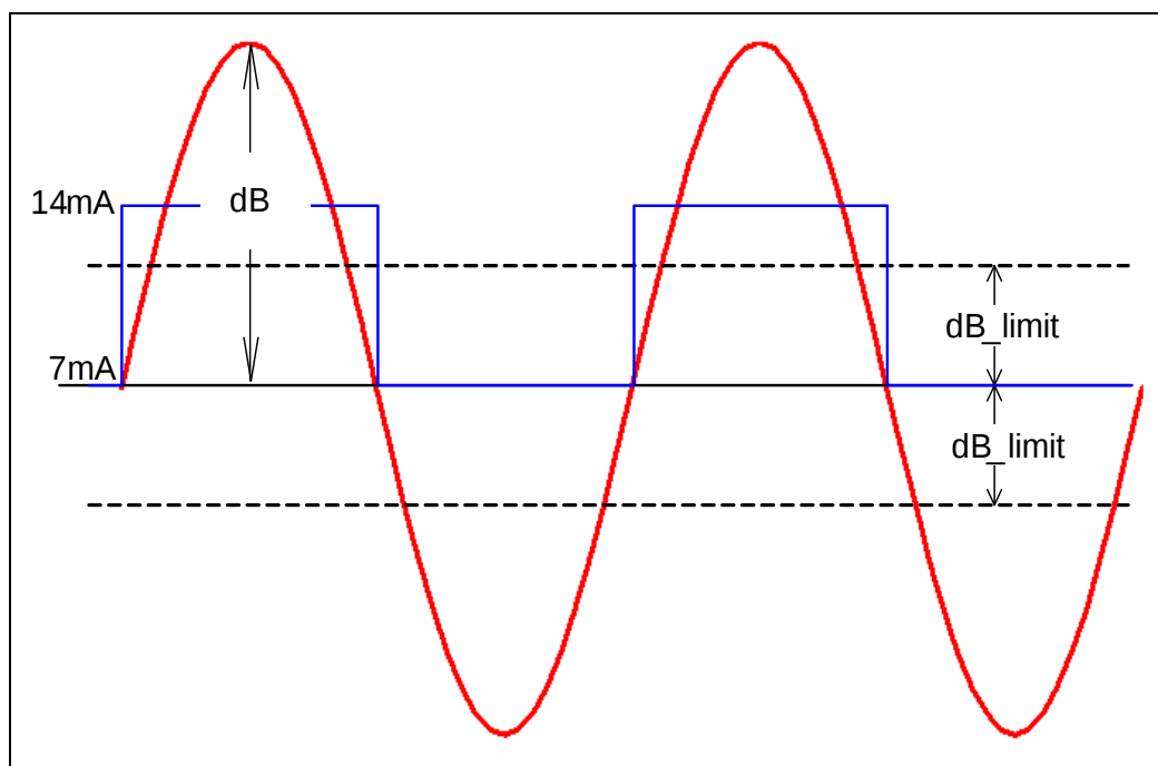
Figure 3-1 Description of differential field dB and switching threshold dB_{\text{limit}} (calibrated mode)
