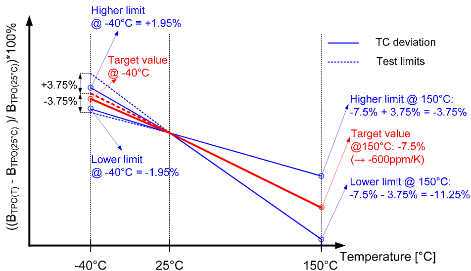
Figure 6: Temperature coefficient of TPO switching point
