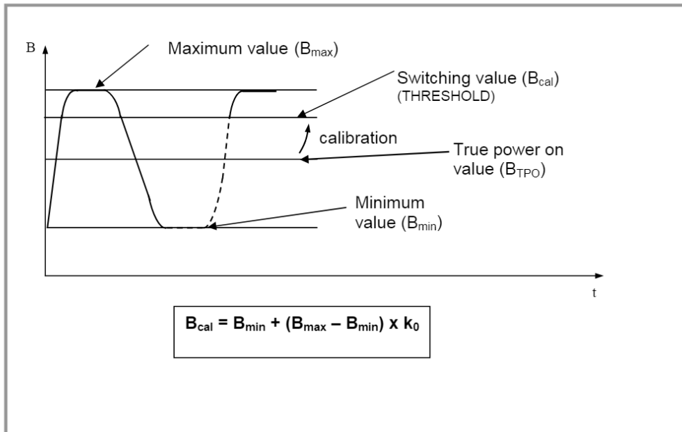
Fig. 4: Dynamic threshold value
