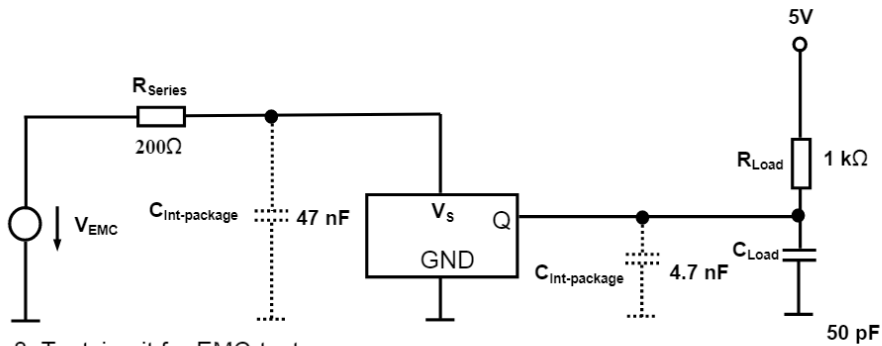
Figure 8: Testcircuit for EMC-tests
