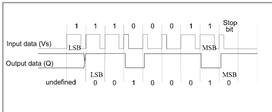
Fig. 5: Serial protocol
