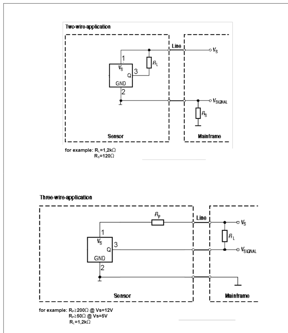
Figure 7 Application Circuits TLE4984C
