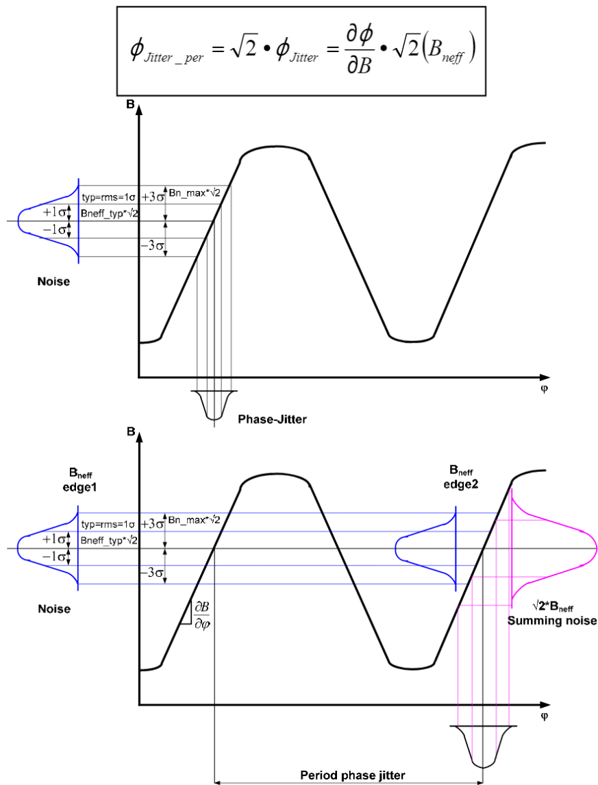
Figure 10: Period phase jitter compared to phase jitter
