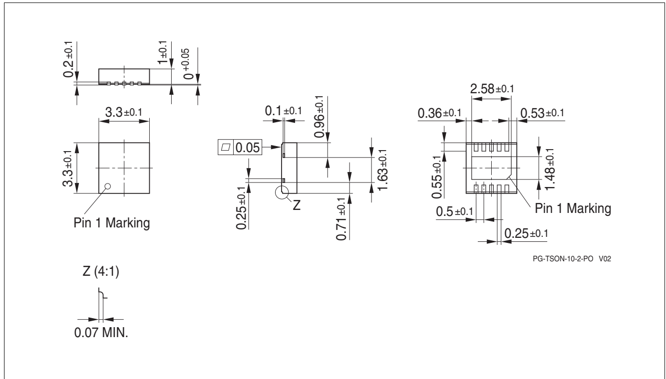
Figure 6 PG-TSON-10
