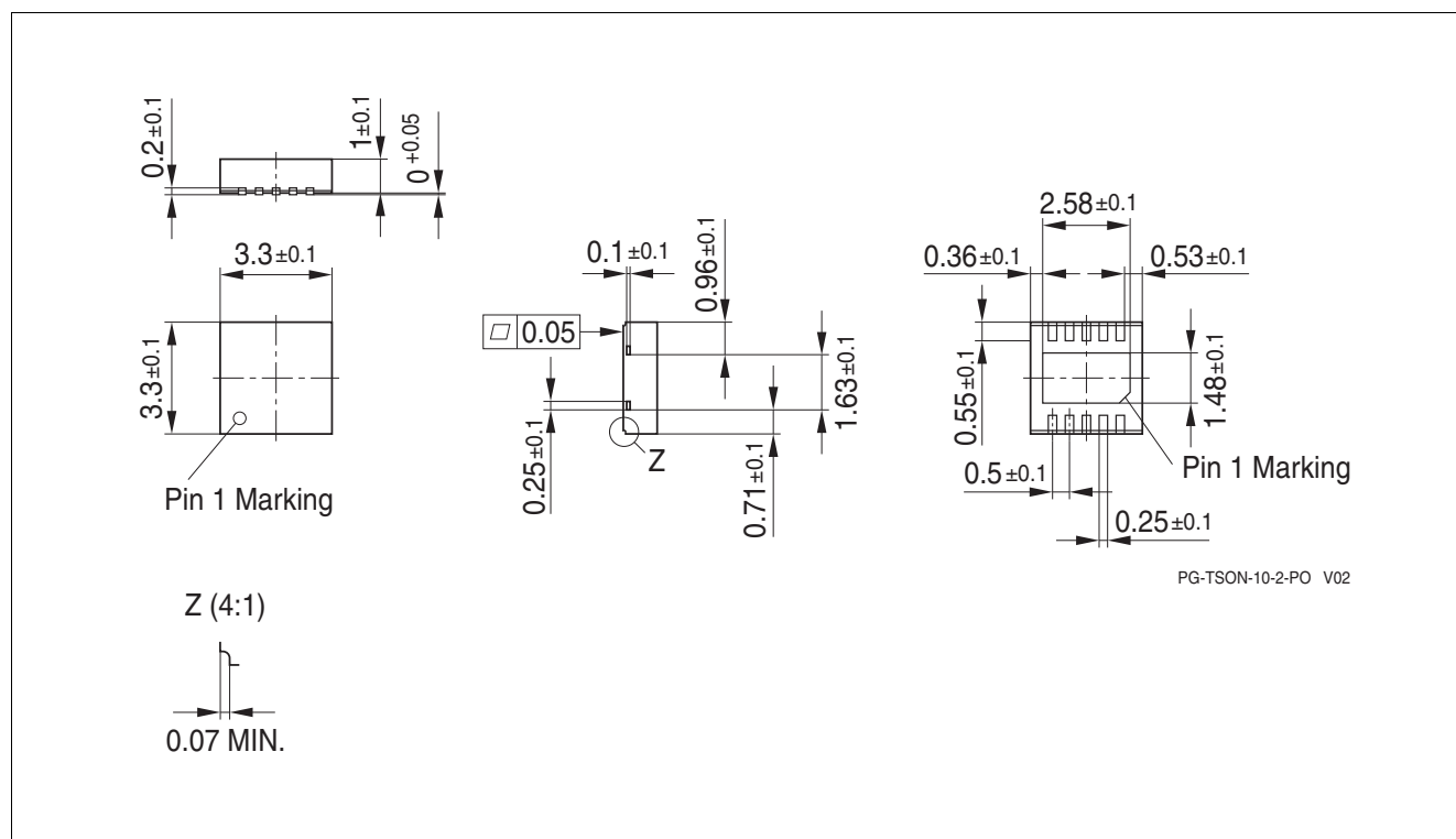
Figure 7 PG-TSON-10
