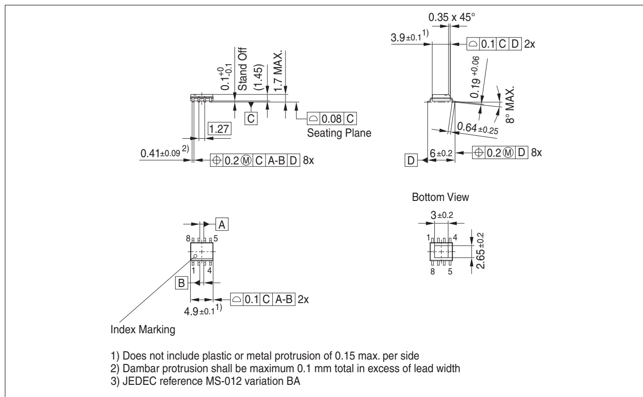
Figure 6 PG-DSO-8 EP
