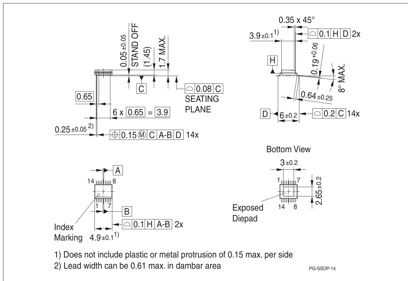
Figure 13 PG-SSOP-14
