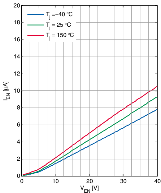
Enable input current I_{\text{EN}} versus enable input voltage V_{\text{EN}}
