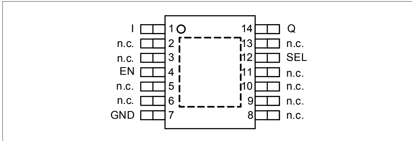
Figure 2 Pin configuration TLS835B2ELVSE
