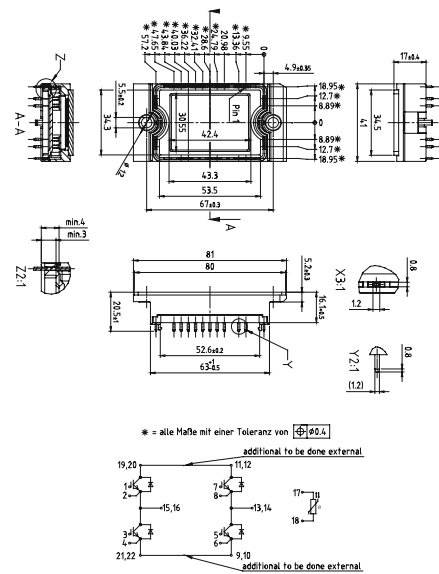
EconoPACK™ 1B FourPACK M_E1c
