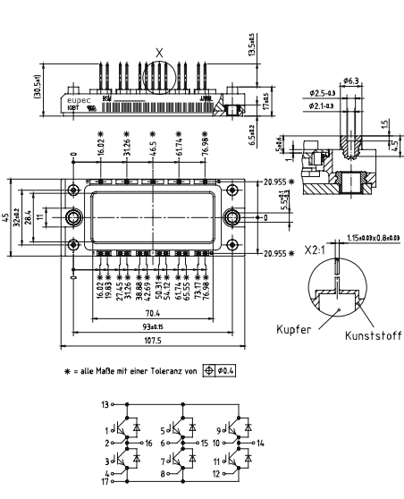
EconoPACK™2 A (longpin) M_E2d
