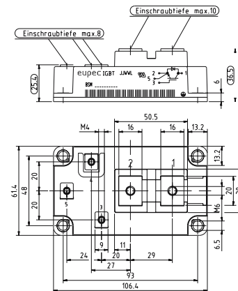
Single Switch 62, collector sense M_62c
