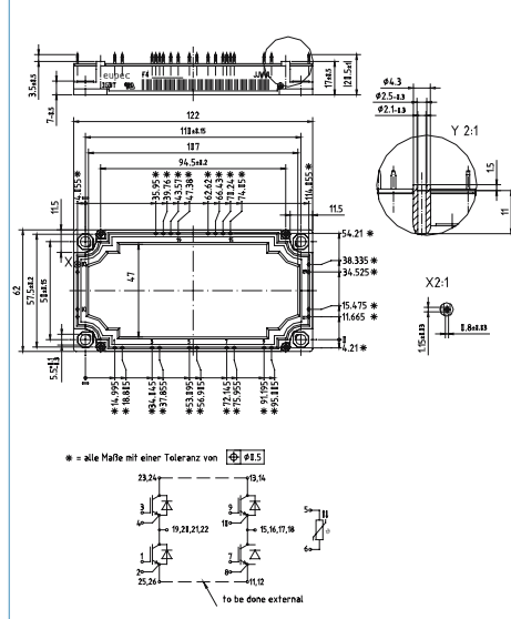
EconoPACK™3 B FourPACK M_E3d
