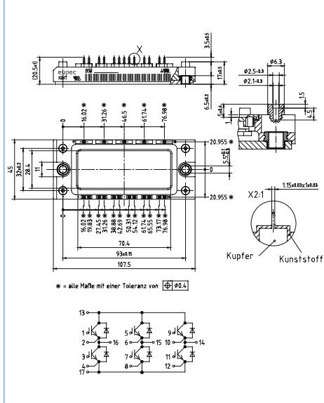
EconoPACK™2 A (shortpin) M_E2c
