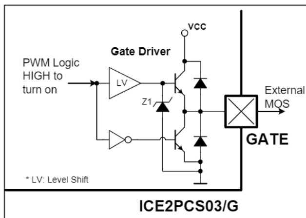
Figure 15 Gate Driver
