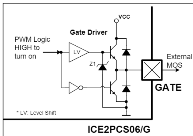
Figure 15 Gate Driver
