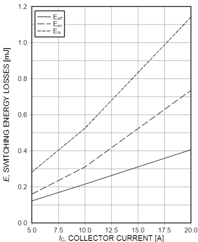
Figure 13. Typical switching energy losses as a function of collector current (inductive load, T_{vj}=175^{\circ}\text{C} , V_{CE}=400\text{V} , V_{GE}=15/0\text{V} , r_G=26\Omega , Dynamic test circuit in Figure E)
