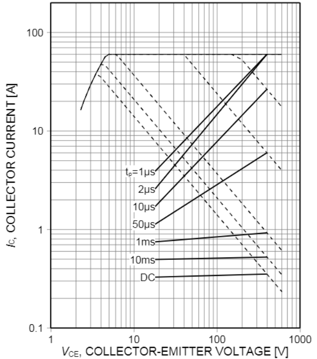
Figure 2. Safe operating area ( D=0 , T_C=25^\circ\text{C} , T_j \leq 150^\circ\text{C} ; V_{GE}=15\text{V} )
