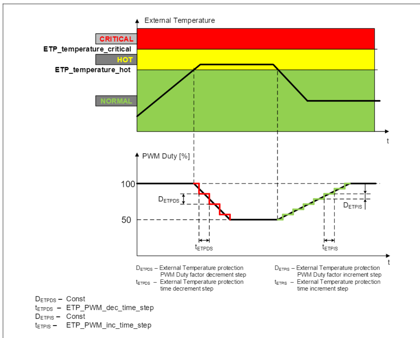
Figure 26. External Temperature Protection Behavior
