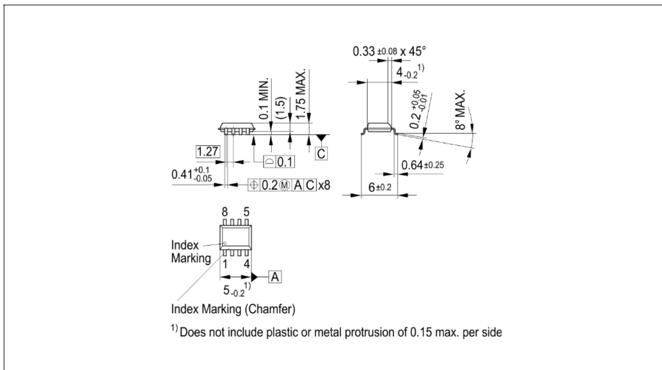
Figure 32. PG-DSO-8-58
