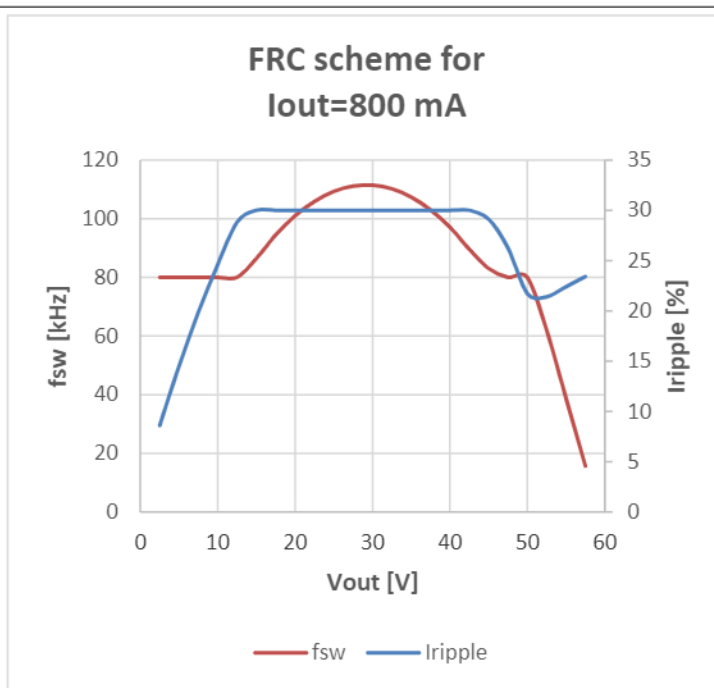
Figure 18. 800 mA FRC Scheme
