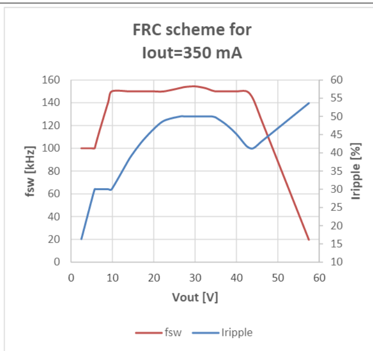
Figure 20. 350 mA FRC Scheme
