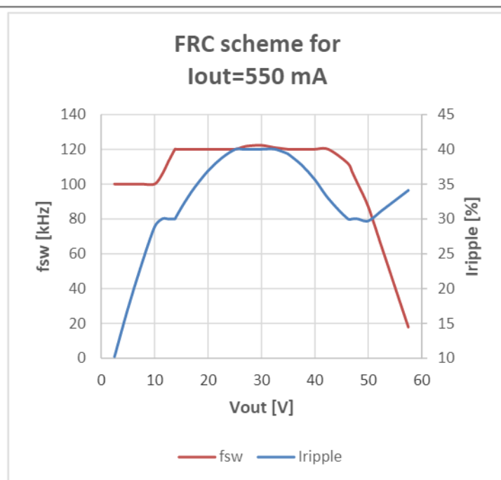
Figure 19. 550 mA FRC Scheme
