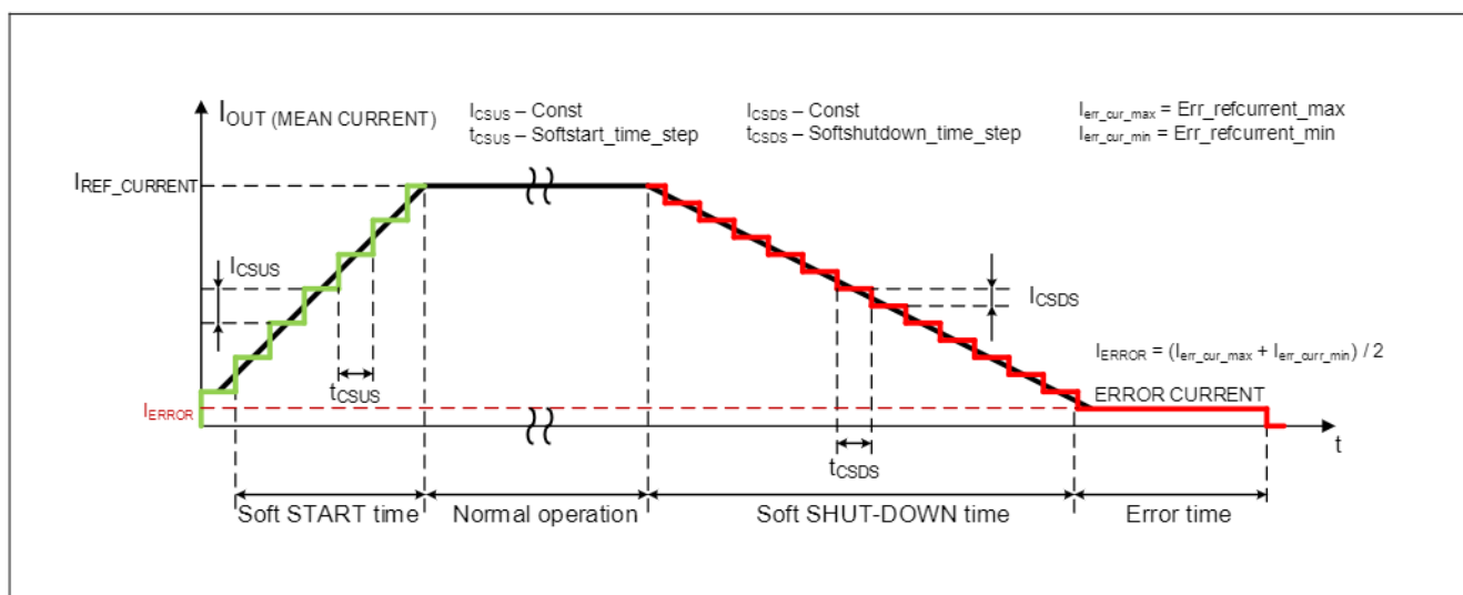
Figure 13. Soft-Start and Soft Shutdown Definitions
