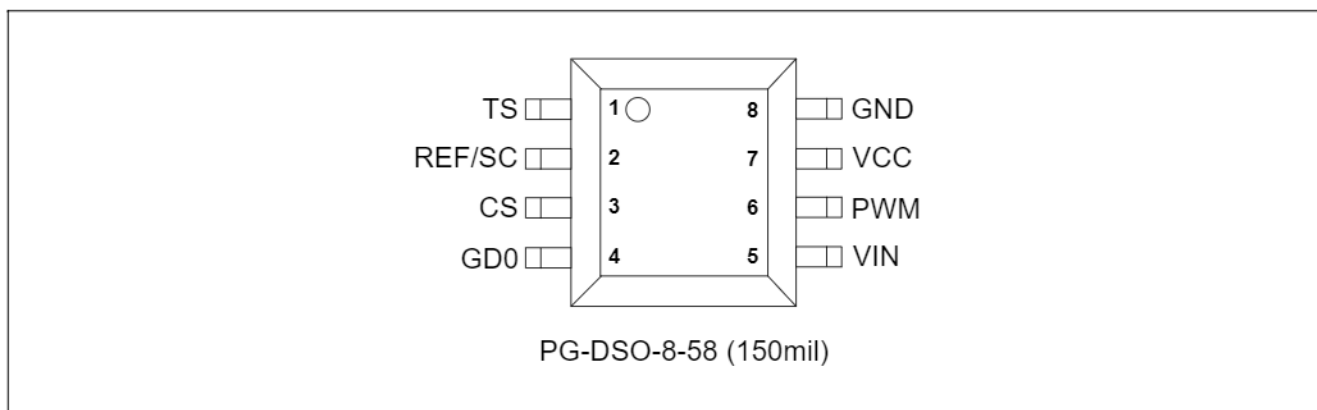
Figure 2. Pin Configuration
