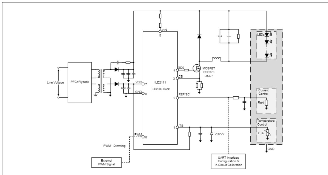
Figure 1. Typical Application
